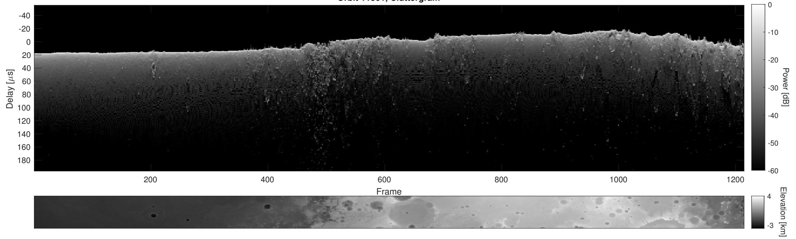
Orbit 11501, Cluttergram
