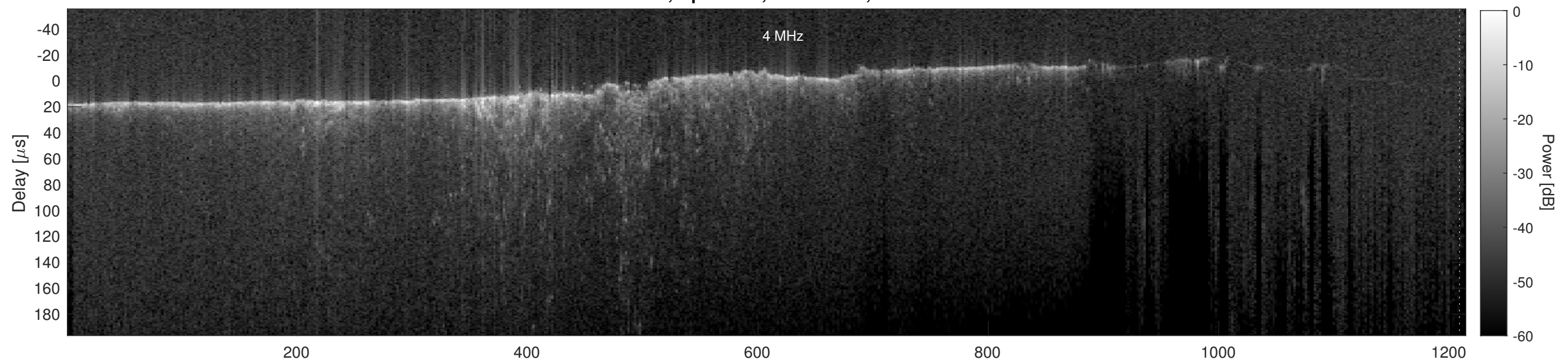
Orbit 11501, Cluttergram
