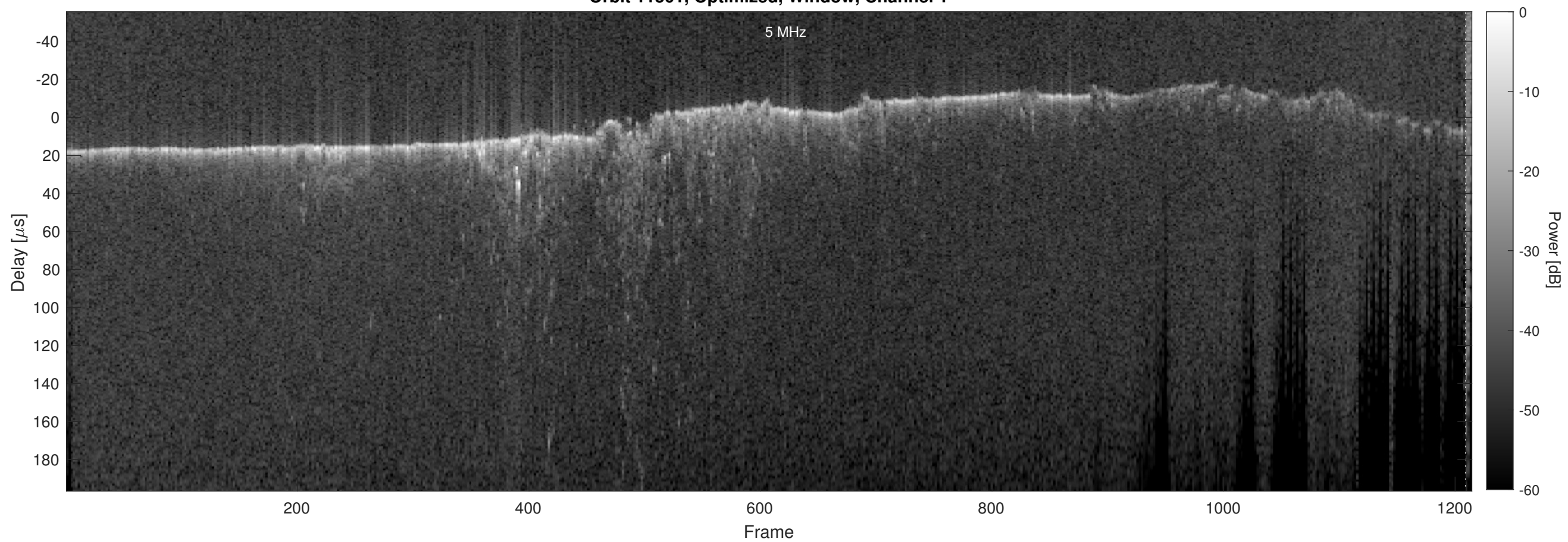
Orbit 11501, Optimized, Window, Channel 2
