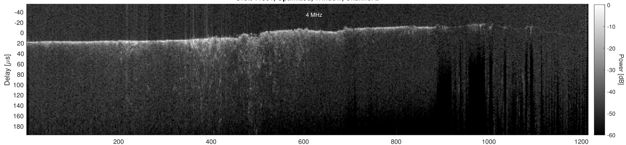
Orbit 11501, Cluttergram
