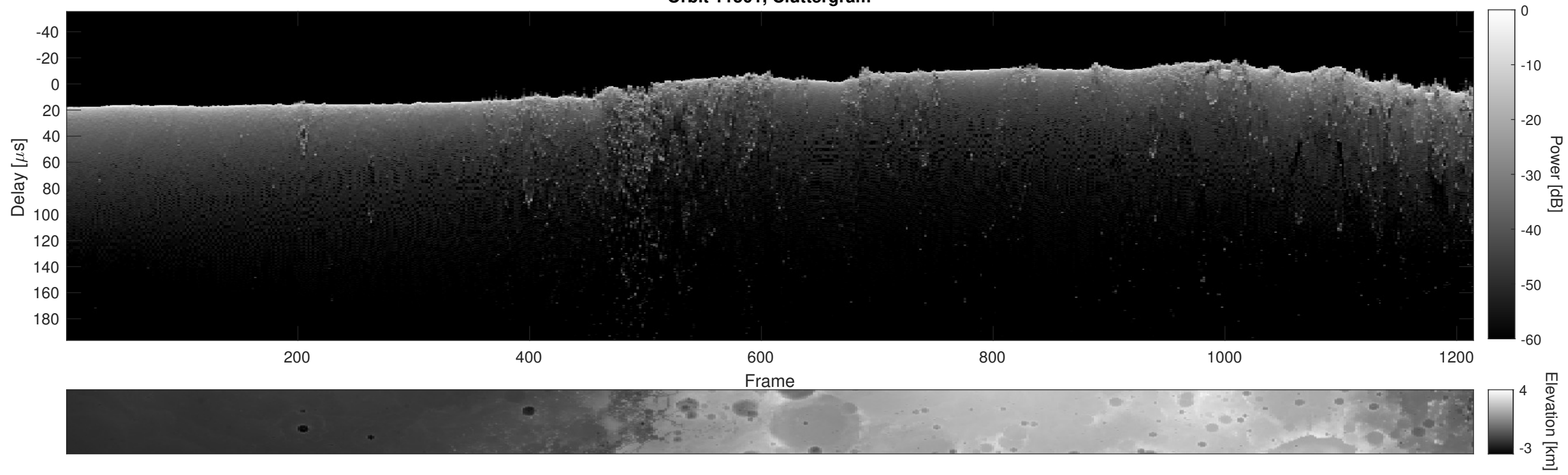
Orbit 11501, Cluttergram
