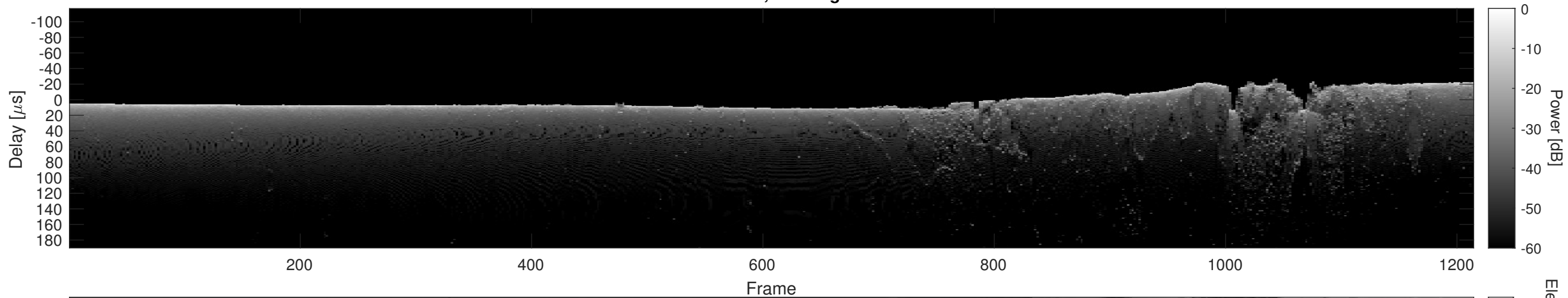
Orbit 11502, Cluttergram
