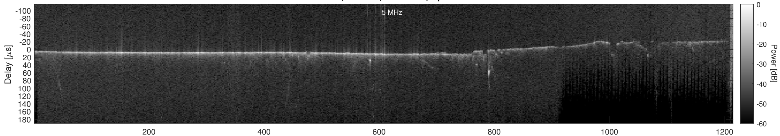
Orbit 11502, Cluttergram
