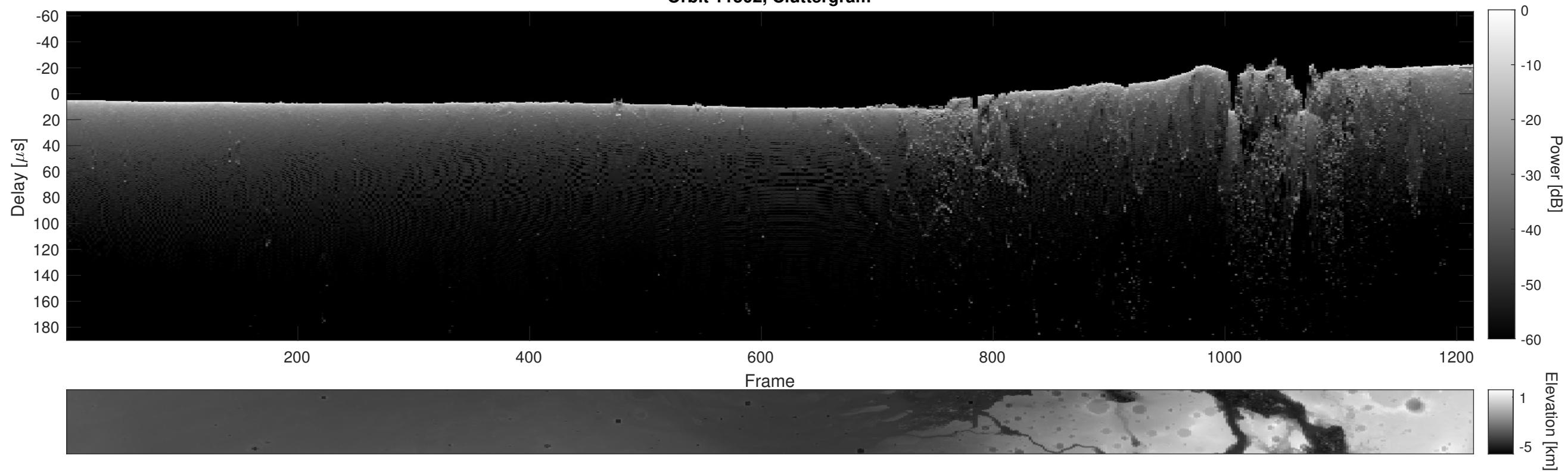
Orbit 11502, Cluttergram
