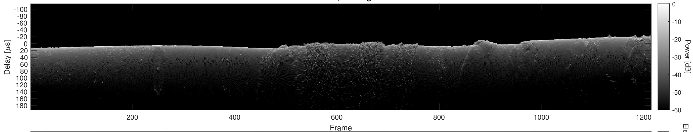
Orbit 11503, Cluttergram
