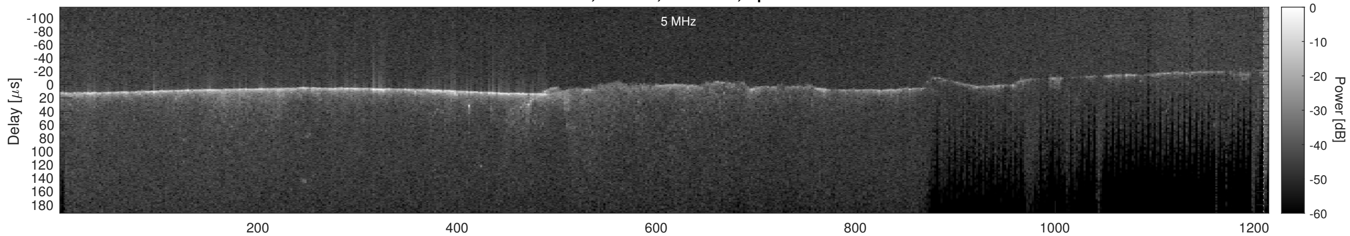
Orbit 11503, Cluttergram
