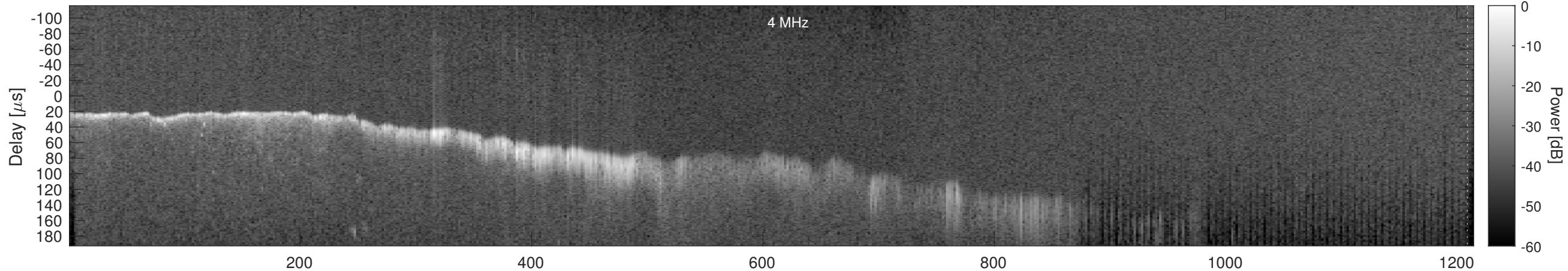
Orbit 11503, Window, Channel 2, Chapman
