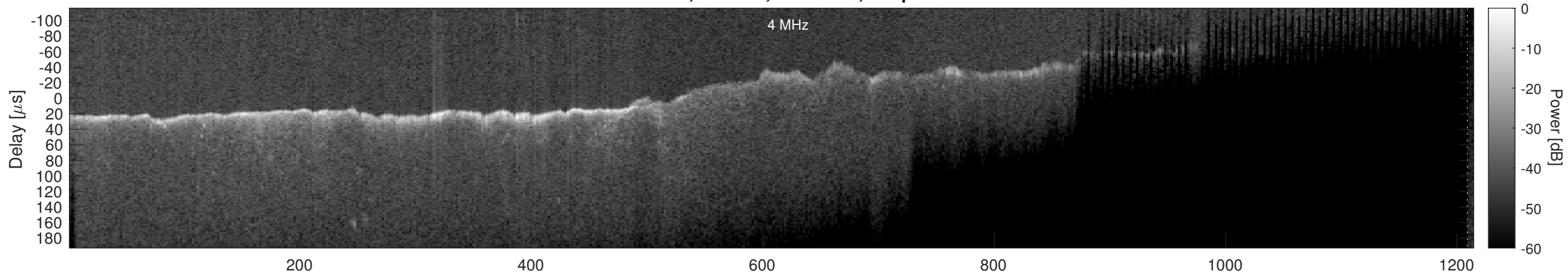
Orbit 11503, Window, Channel 2, Optimized
