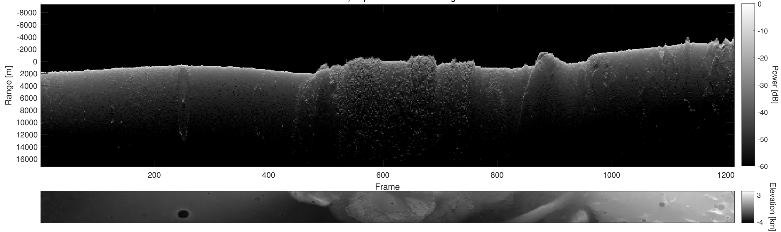
Orbit 11503, Depth-Corrected Cluttergram
