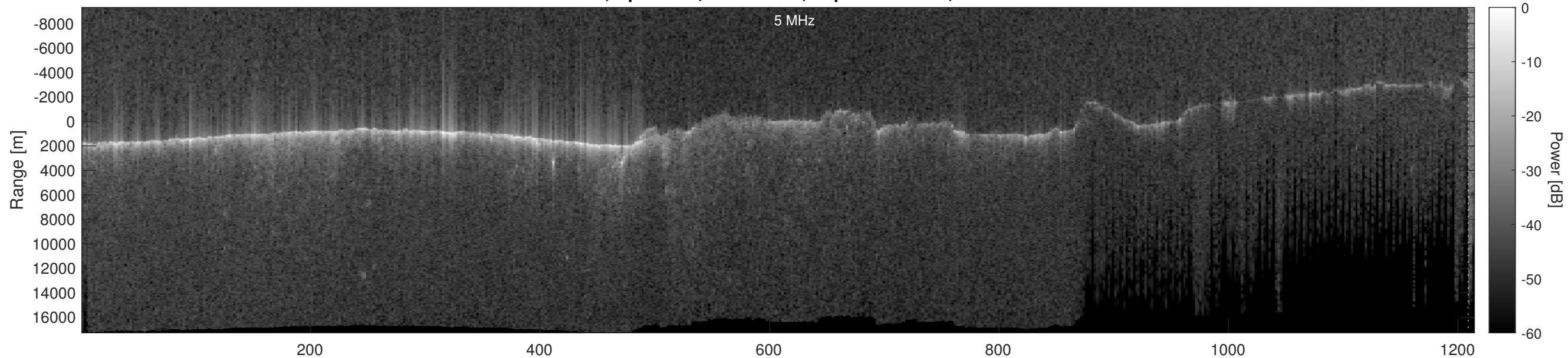
Orbit 11503, Optimized, No Window, Depth-Corrected, Channel 2
