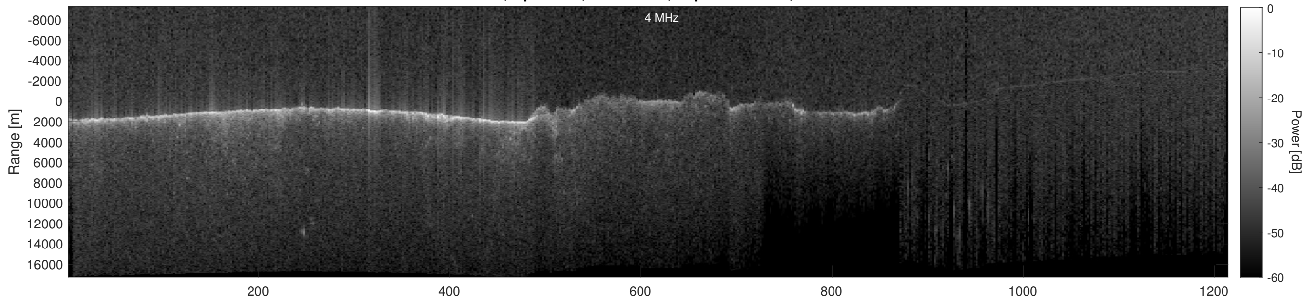
Orbit 11503, Depth-Corrected Cluttergram
