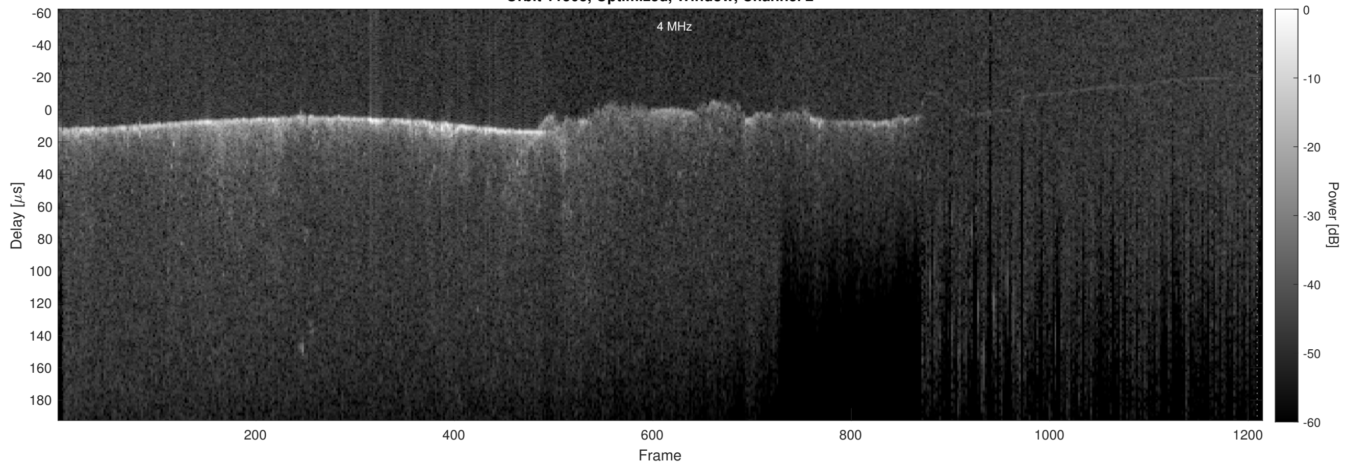
Orbit 11503, Optimized, Window, Channel 2
