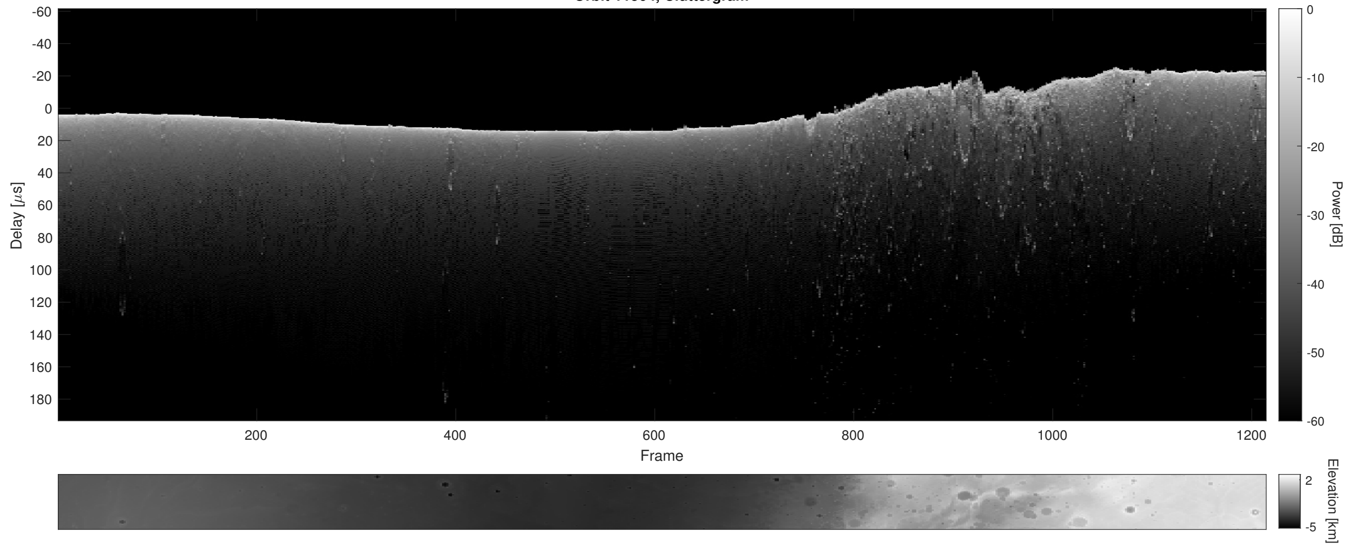
Orbit 11504, Cluttergram
