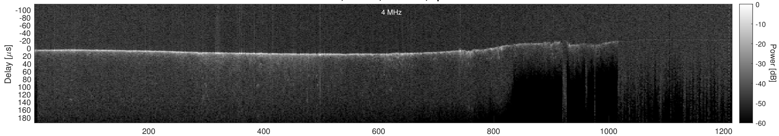
Orbit 11504, Cluttergram
