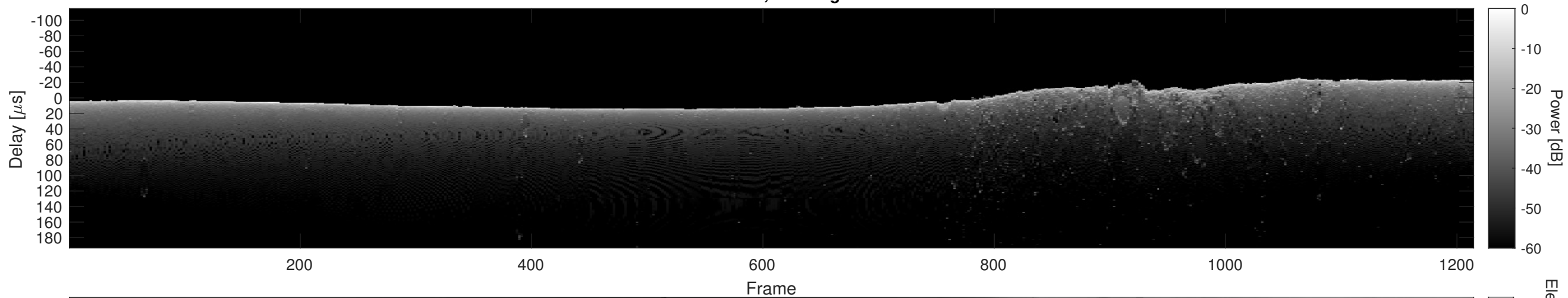
Orbit 11504, Cluttergram
