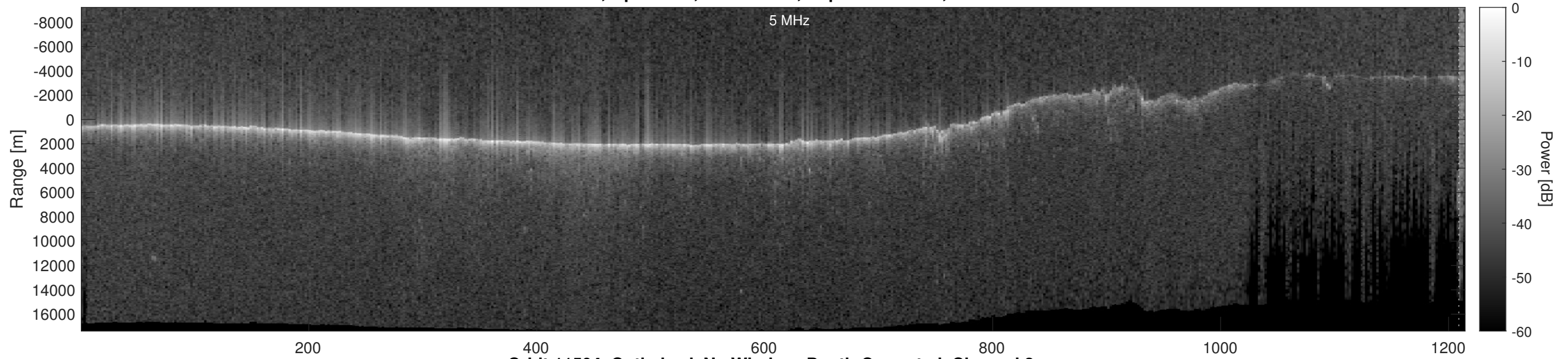
Orbit 11504, Optimized, No Window, Depth-Corrected, Channel 2
