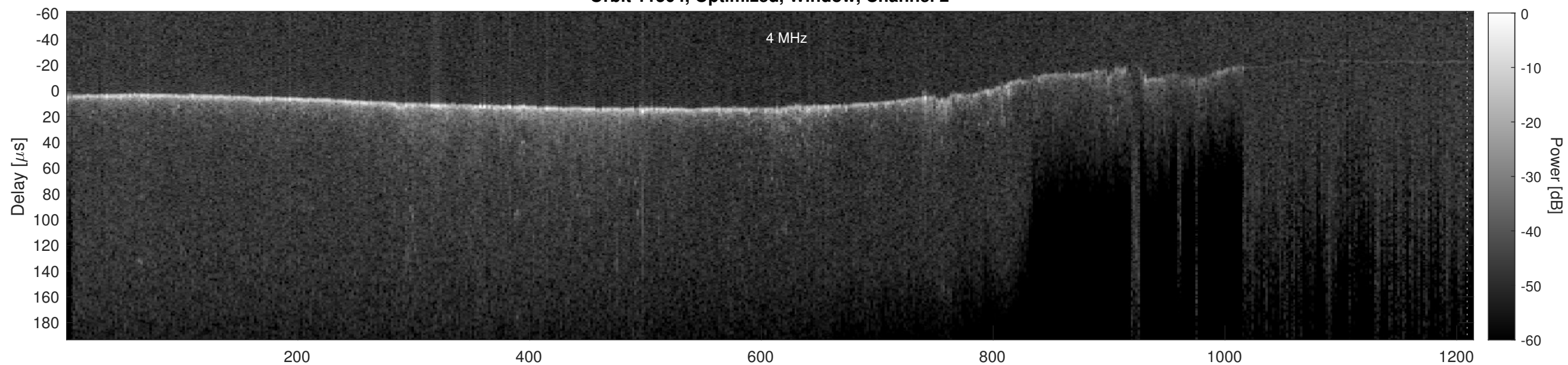
Orbit 11504, Cluttergram
