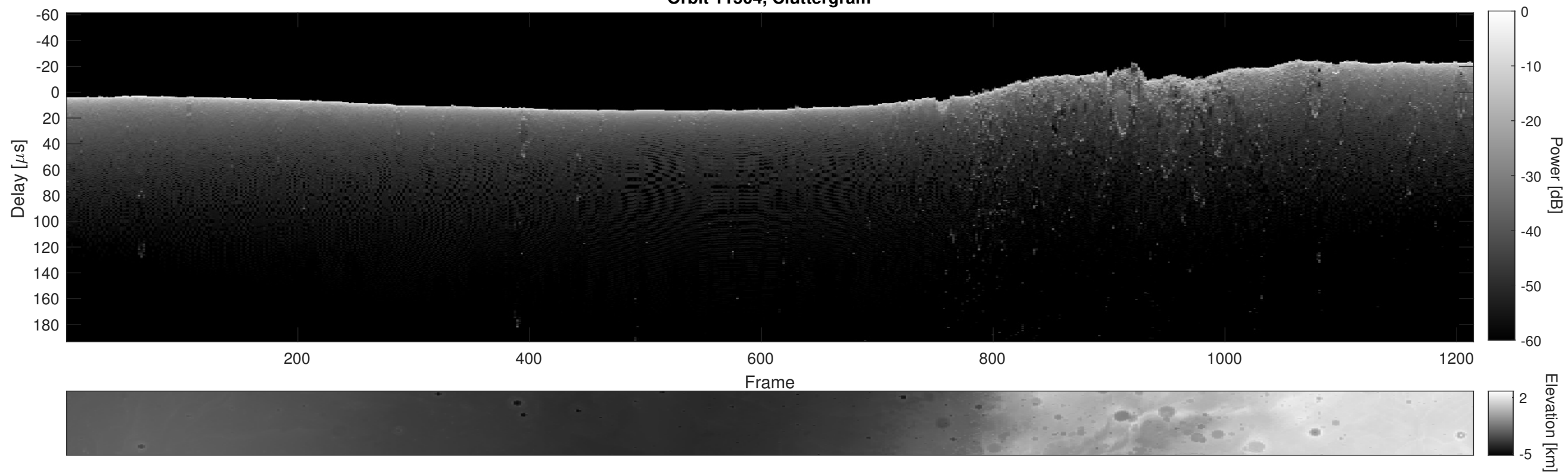
Orbit 11504, Cluttergram
