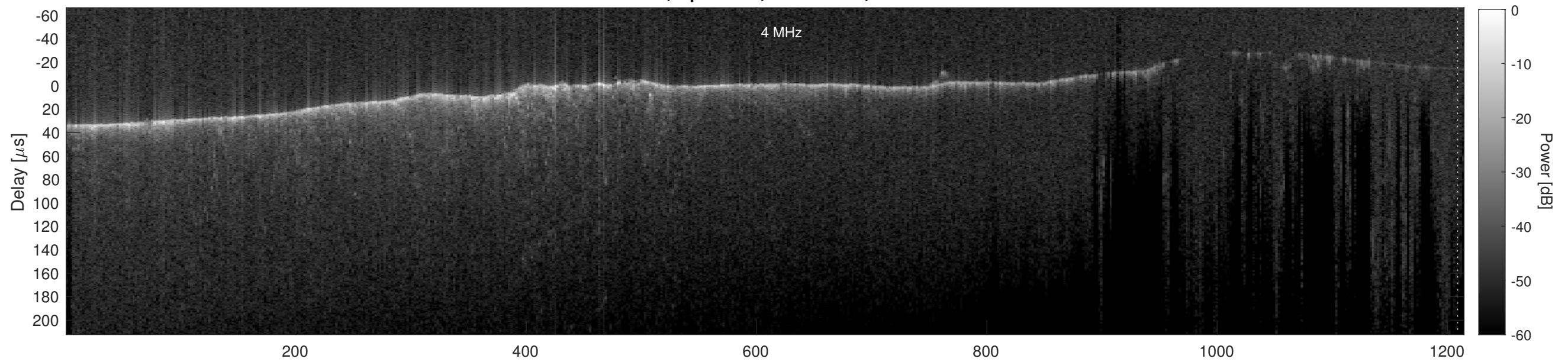
Orbit 11506, Cluttergram
