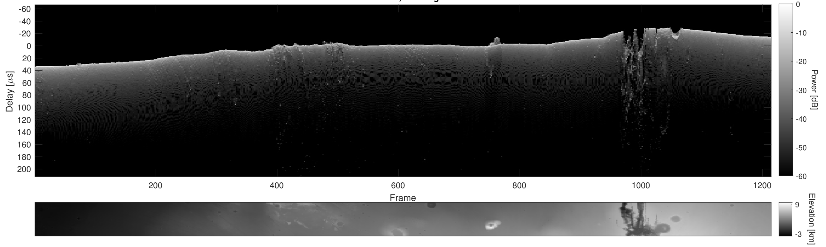
Orbit 11506, Cluttergram
