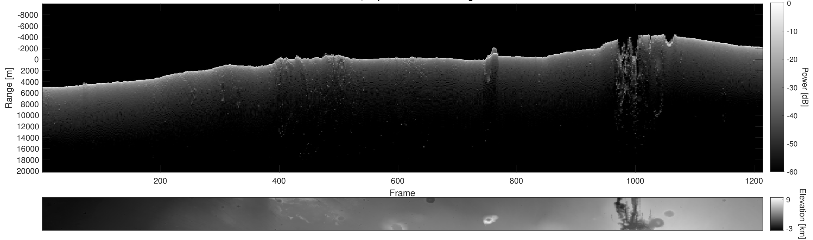
Orbit 11506, Depth-Corrected Cluttergram
