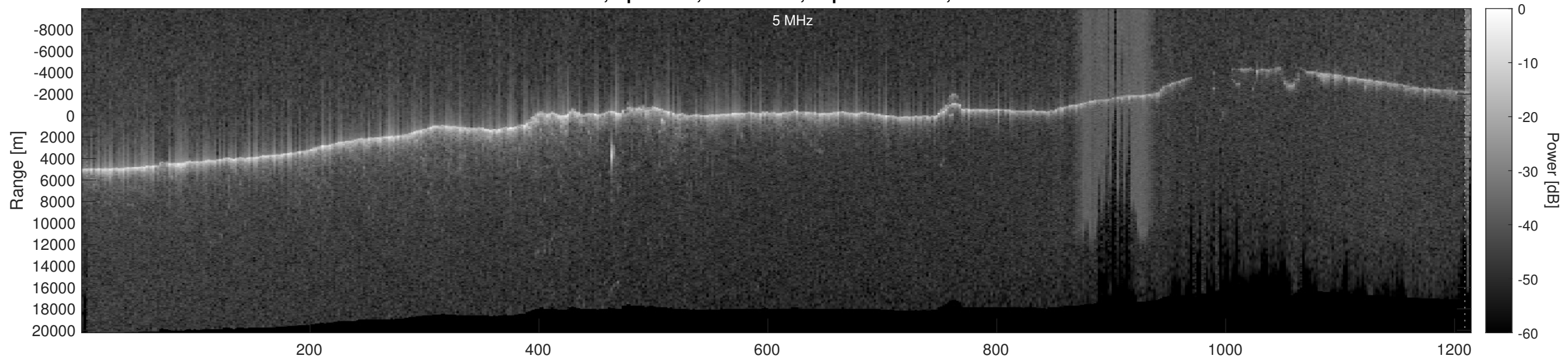
Orbit 11506, Optimized, No Window, Depth-Corrected, Channel 2
