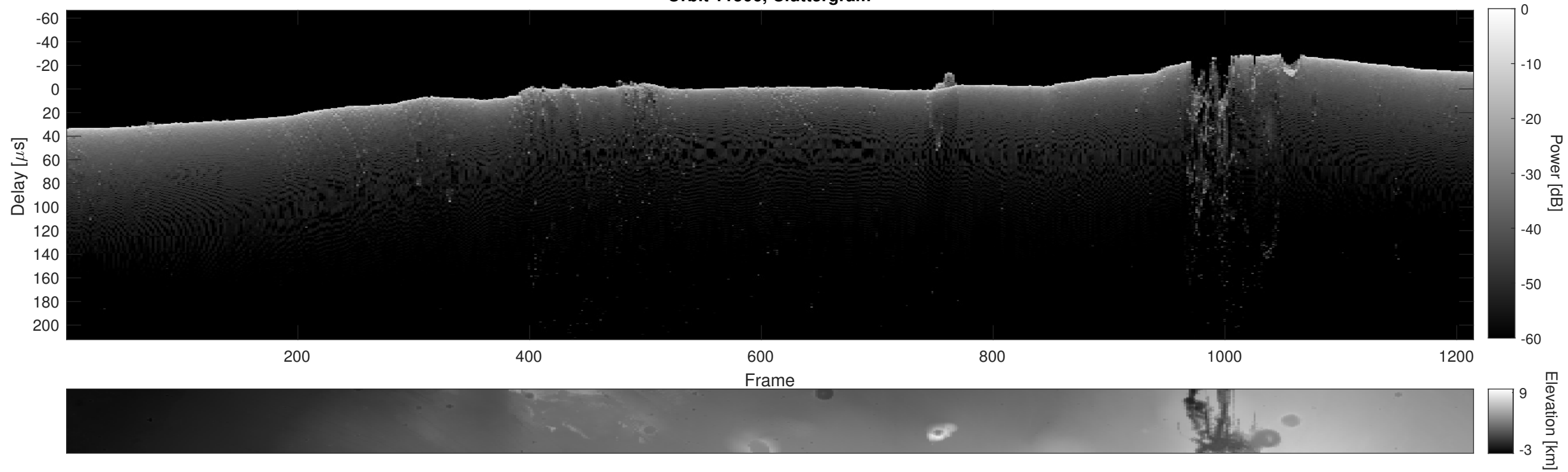
Orbit 11506, Cluttergram
