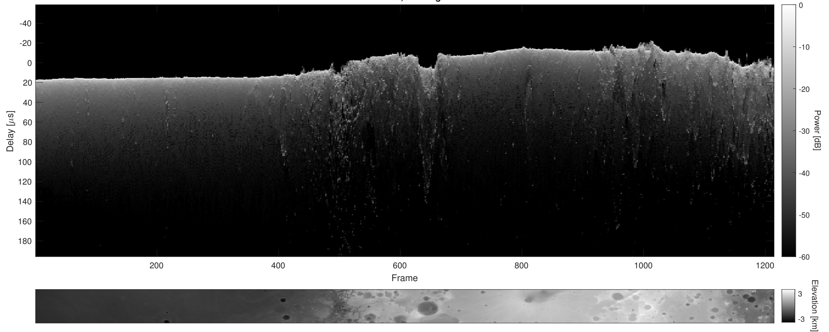
Orbit 11508, Cluttergram
