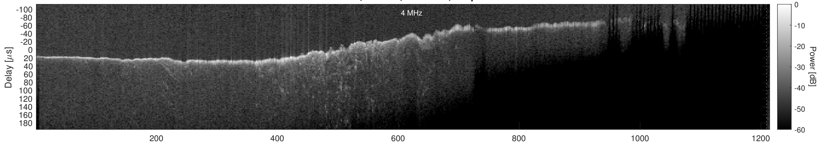
Orbit 11508, Window, Channel 2, Optimized
