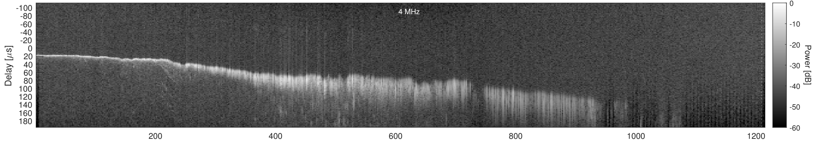
Orbit 11508, Window, Channel 2, Chapman
