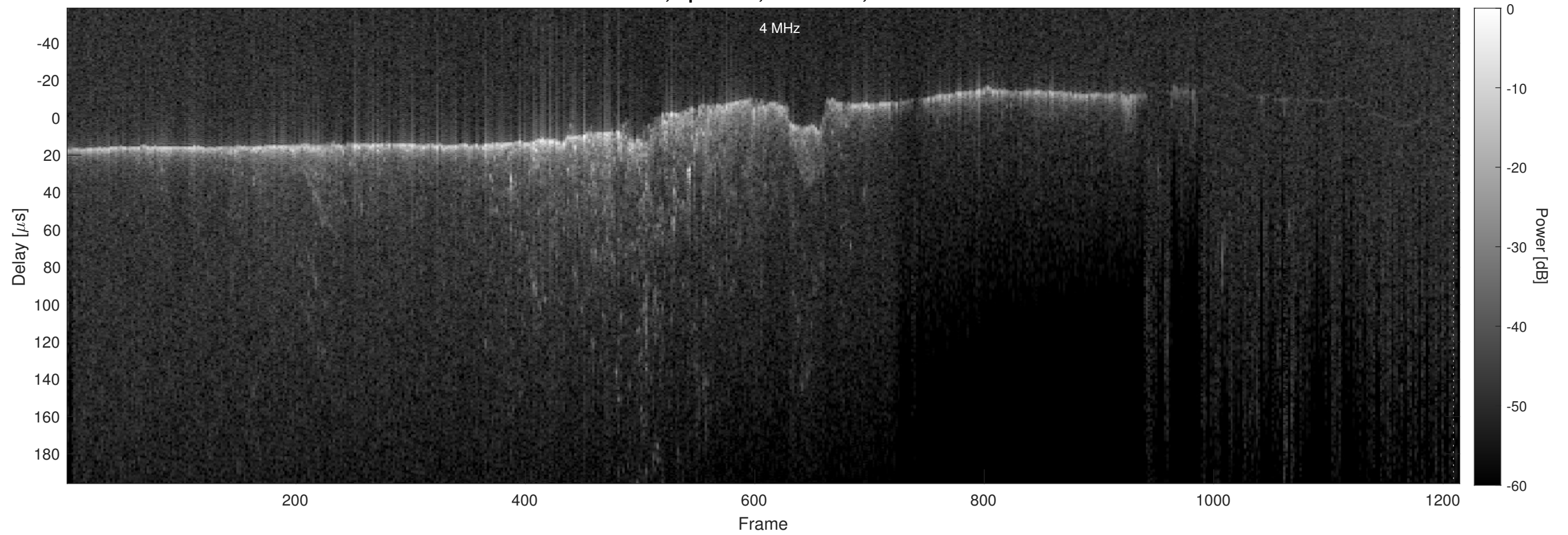
Orbit 11508, Optimized, No Window, Channel 2
