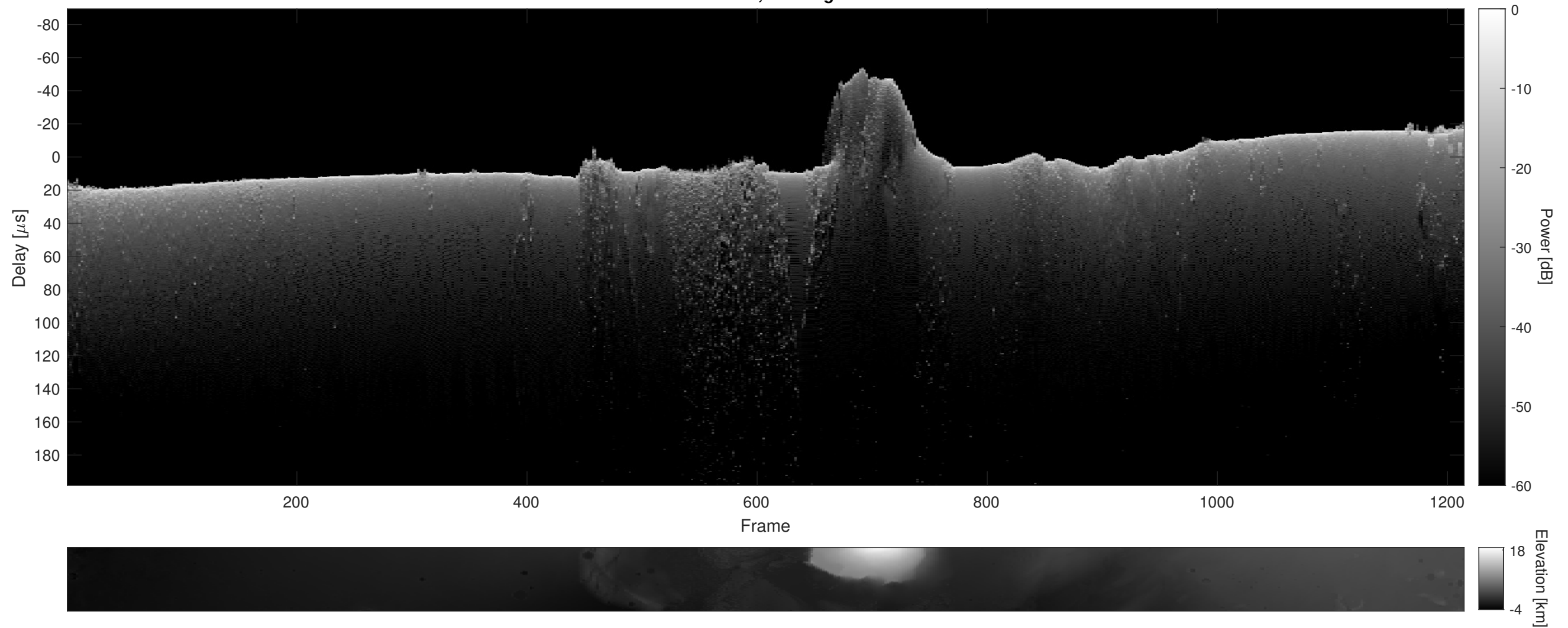
Orbit 11510, Cluttergram
