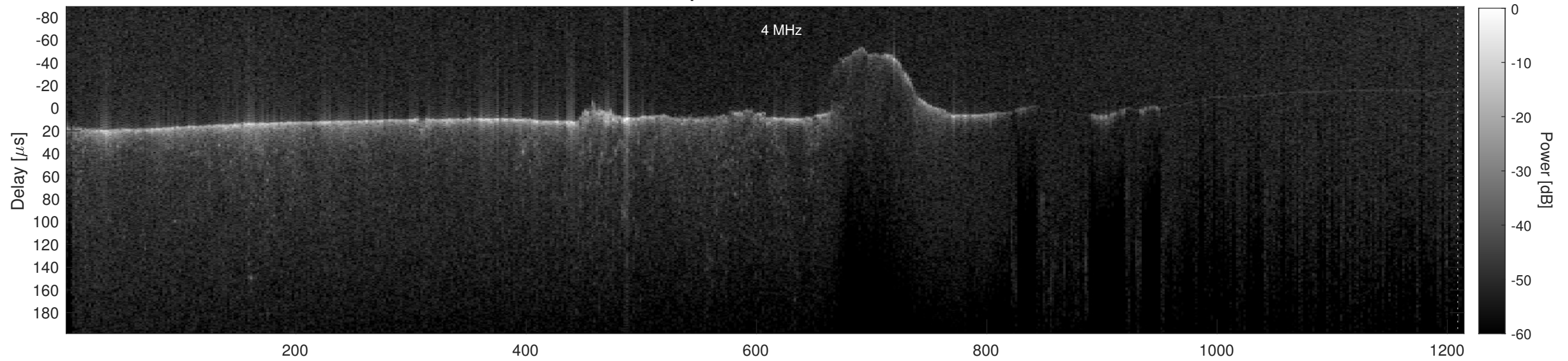
Orbit 11510, Cluttergram
