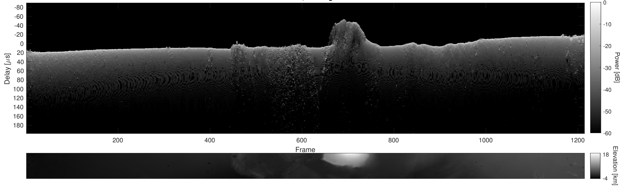
Orbit 11510, Cluttergram
