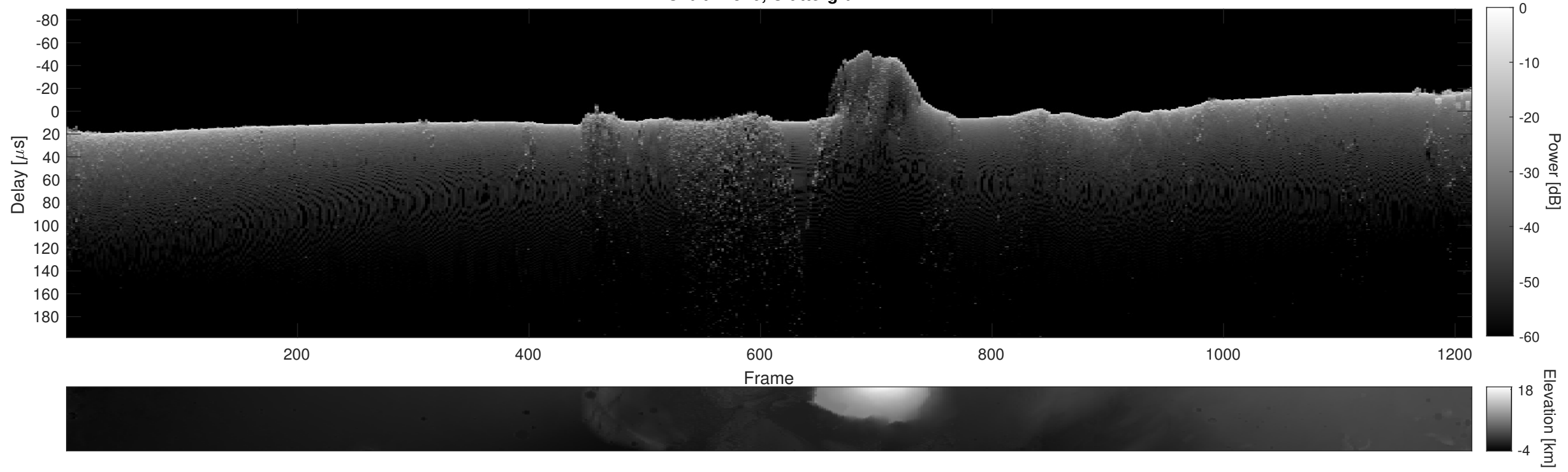
Orbit 11510, Cluttergram
