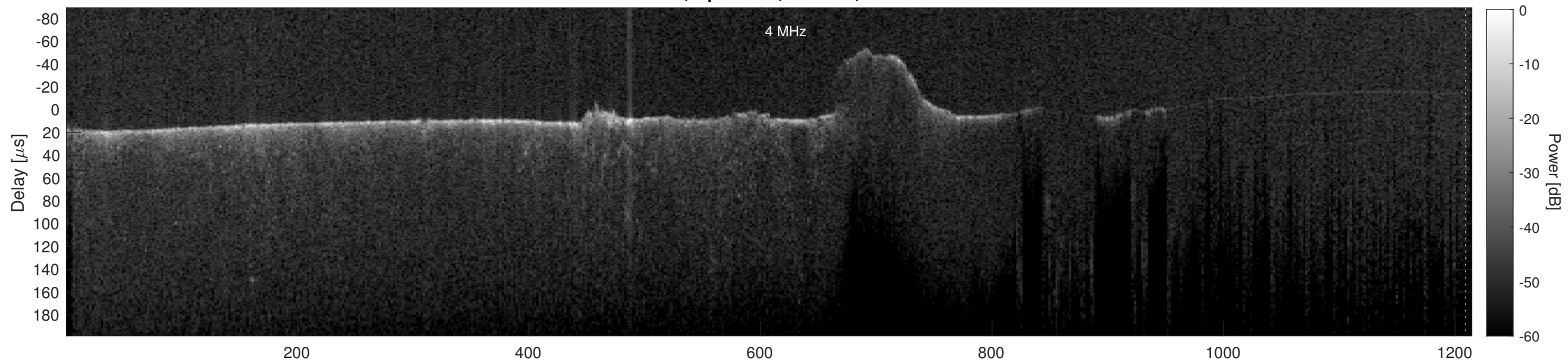
Orbit 11510, Cluttergram
