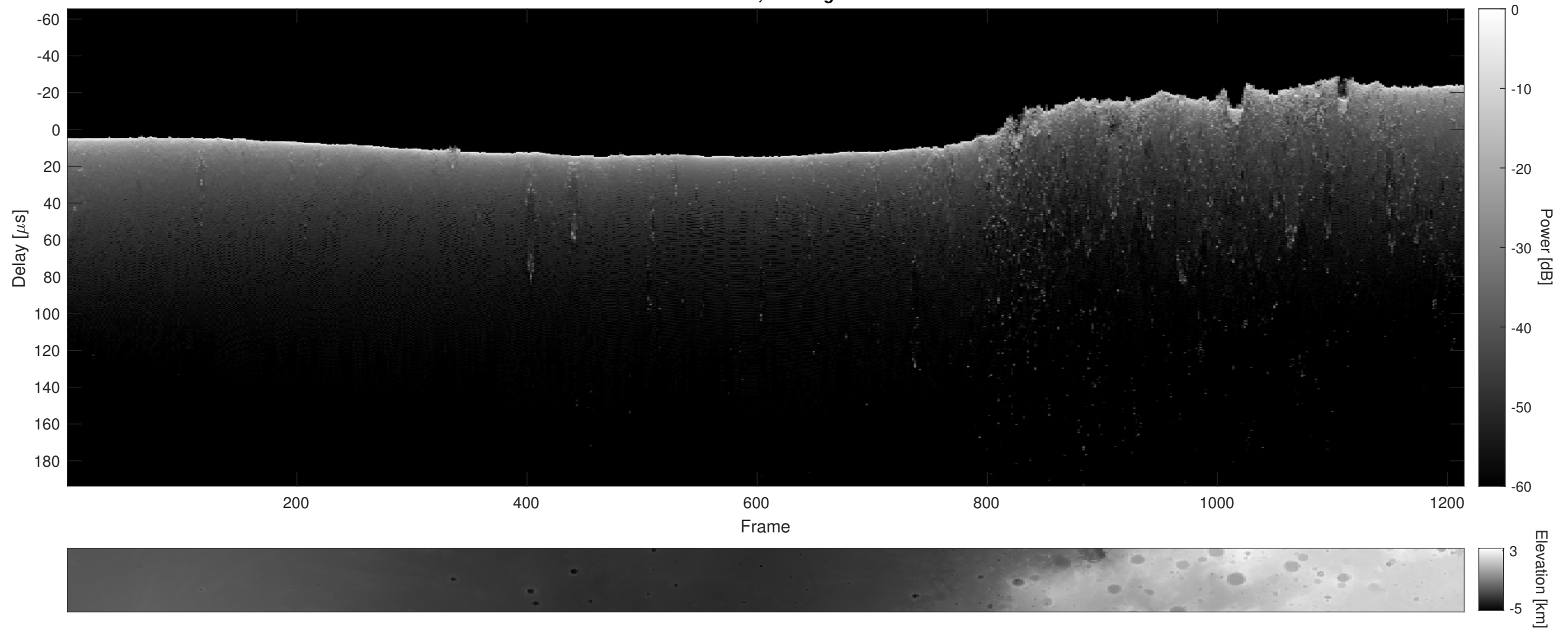
Orbit 11511, Cluttergram
