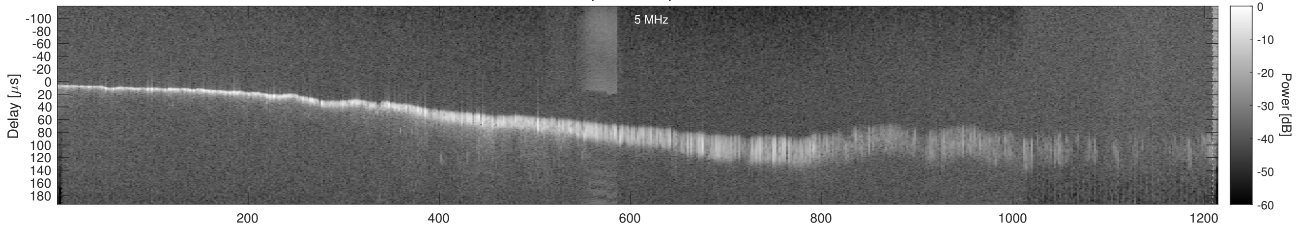
Orbit 11511, Window, Channel 1, Chapman
