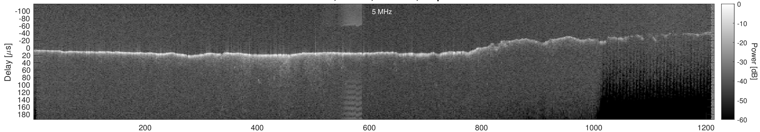
Orbit 11511, Window, Channel 1, Optimized
