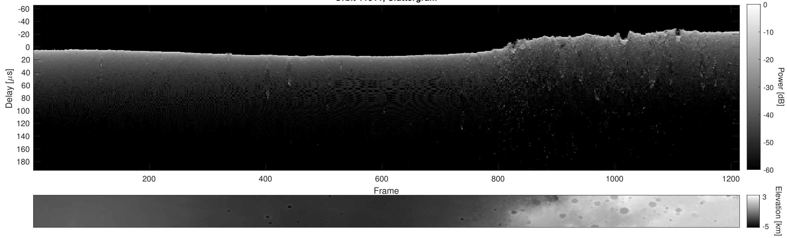
Orbit 11511, Cluttergram
