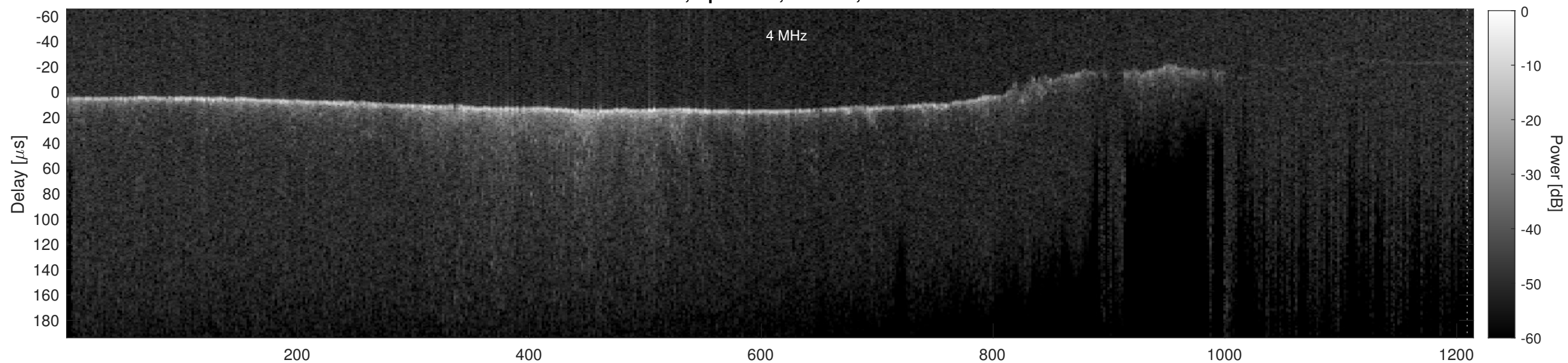
Orbit 11511, Cluttergram
