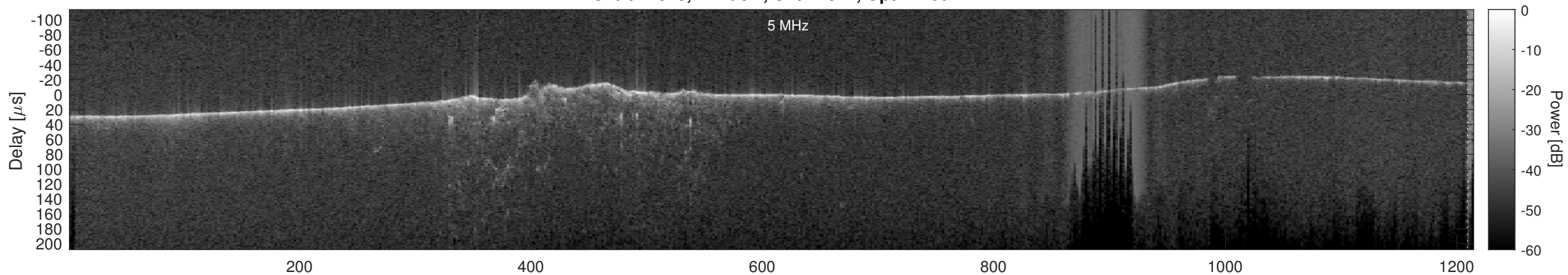
Orbit 11513, Cluttergram
