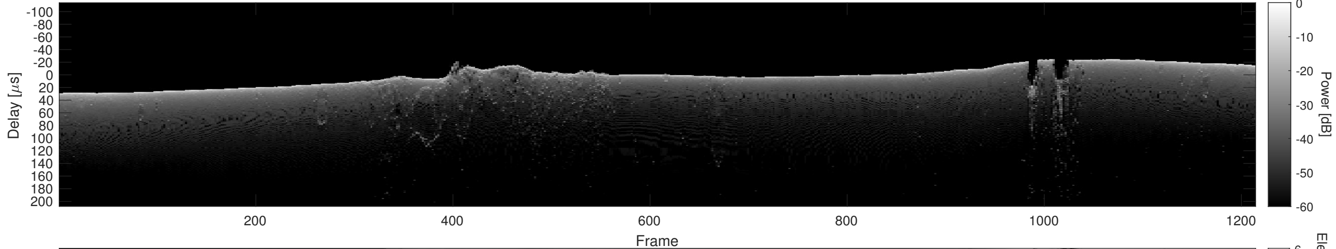
Orbit 11513, Cluttergram
