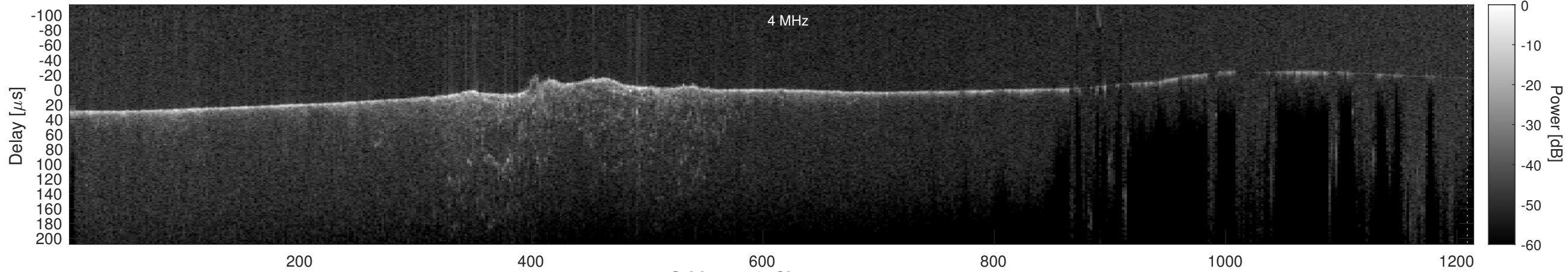
Orbit 11513, Cluttergram
