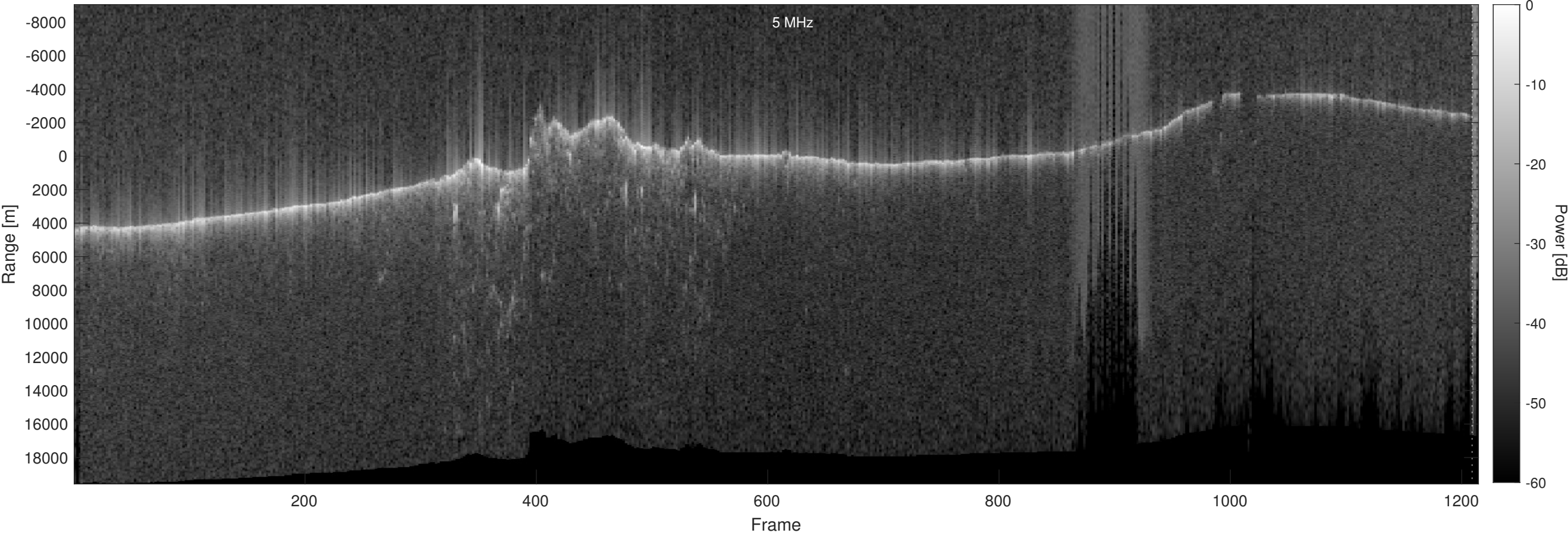
Orbit 11513, Optimized, No Window, Depth-Corrected, Channel 2
