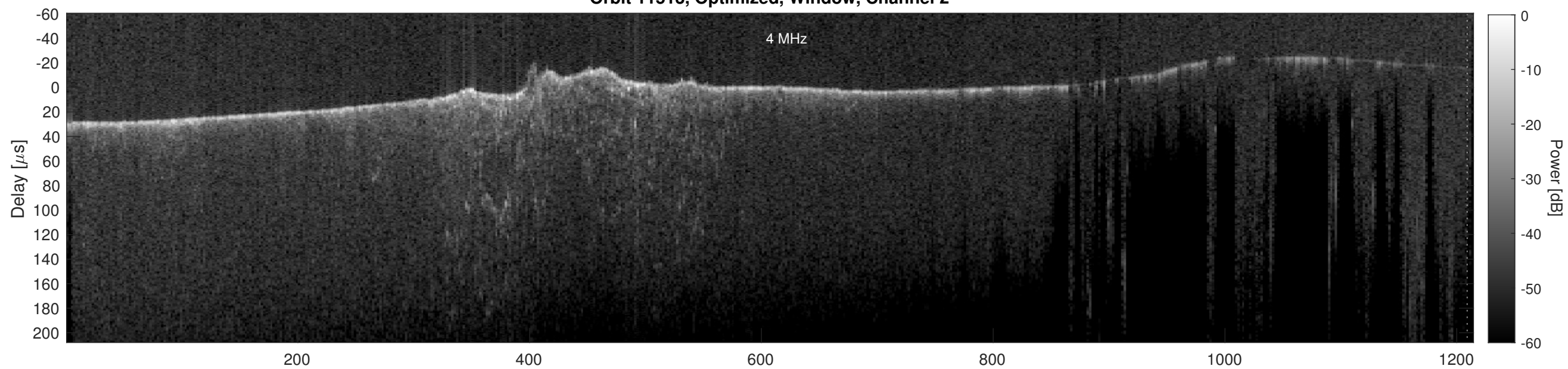
Orbit 11513, Cluttergram
