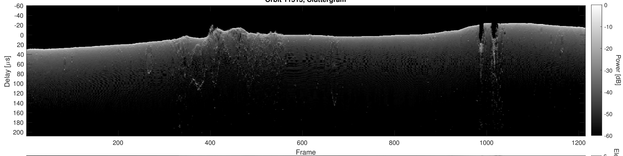
Orbit 11513, Cluttergram
