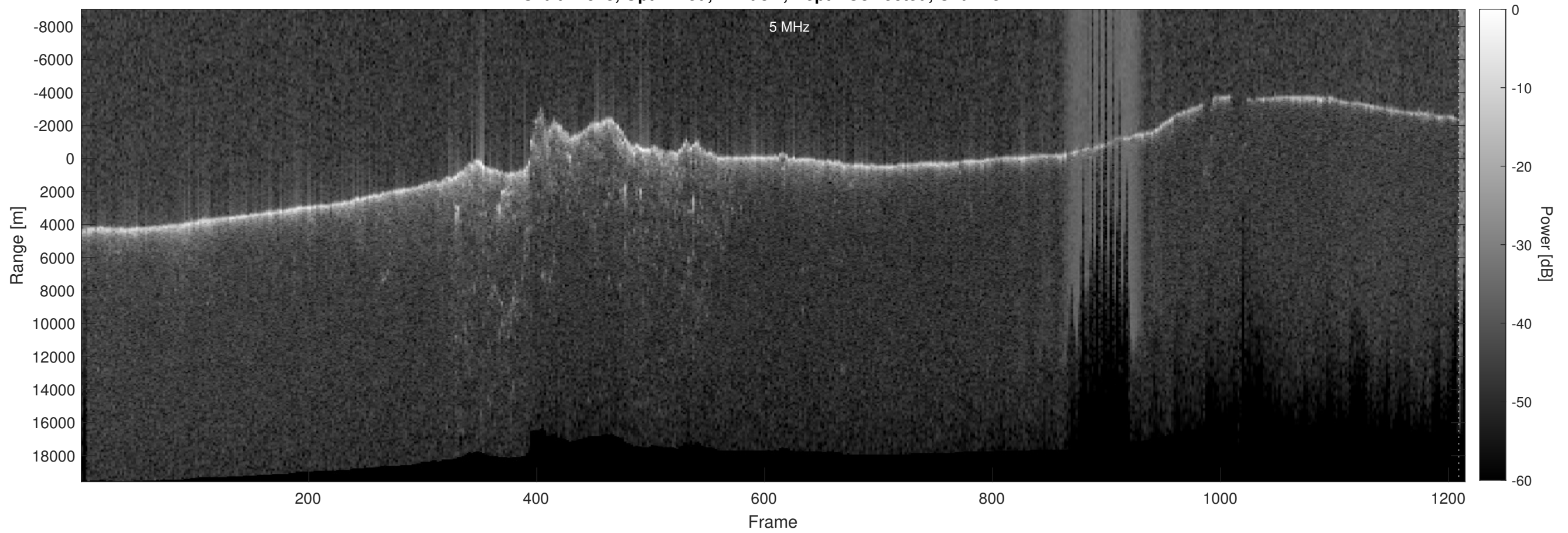
Orbit 11513, Optimized, Window, Depth-Corrected, Channel 2
