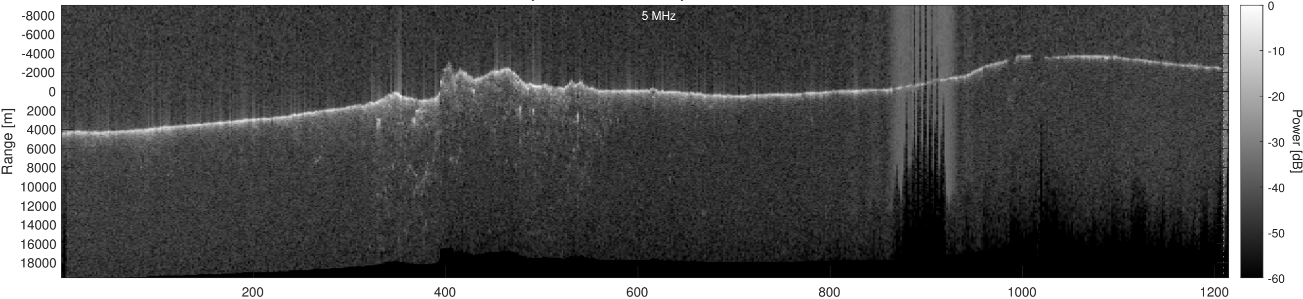
Orbit 11513, Optimized, Window, Depth-Corrected, Channel 2
