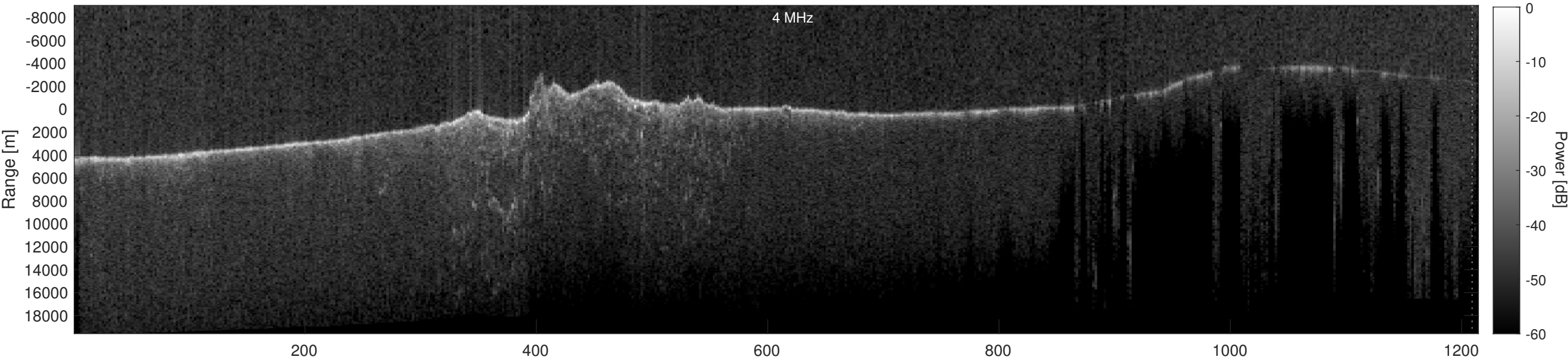
Orbit 11513, Depth-Corrected Cluttergram
