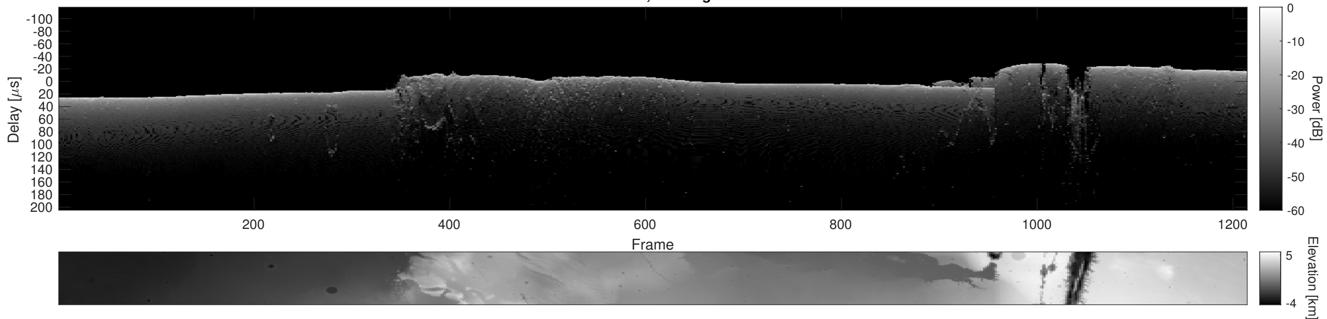
Orbit 11520, Cluttergram
