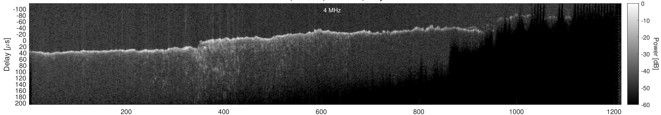
Orbit 11520, Window, Channel 2, Optimized
