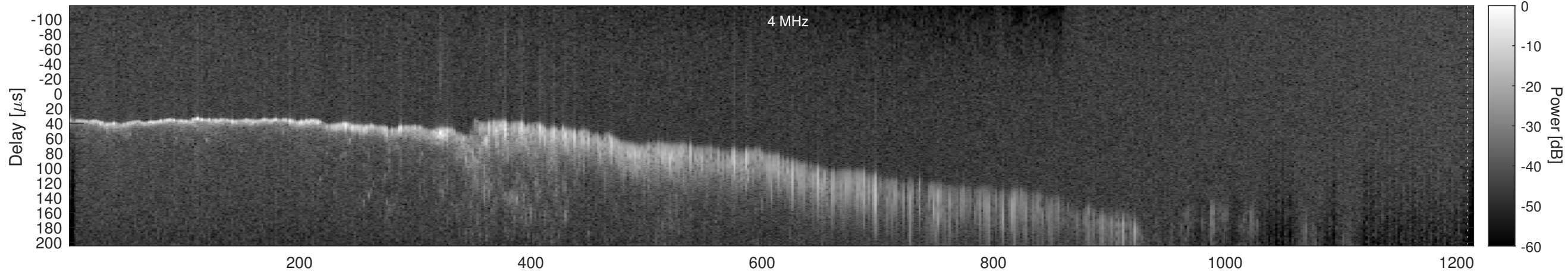
Orbit 11520, Window, Channel 2, Chapman
