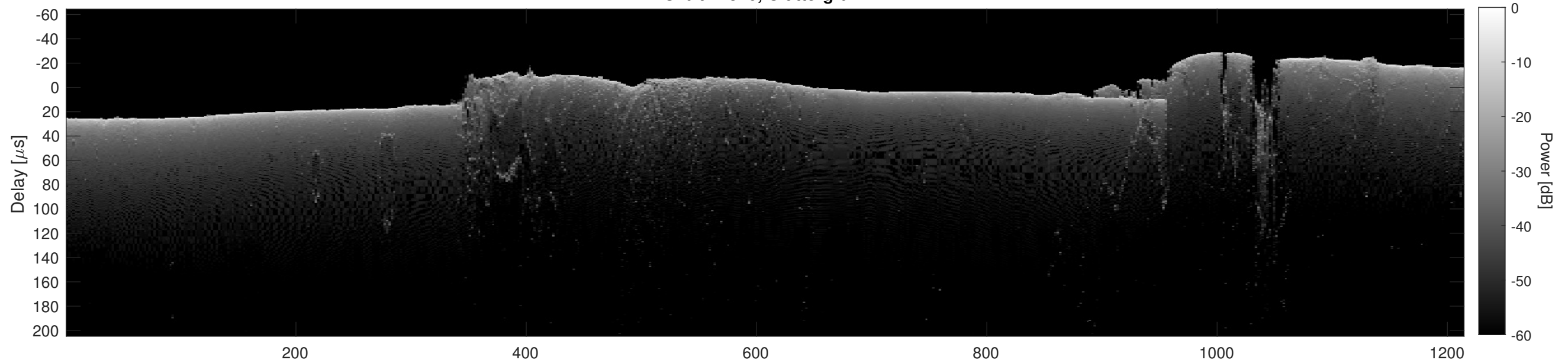
Orbit 11520, Cluttergram
