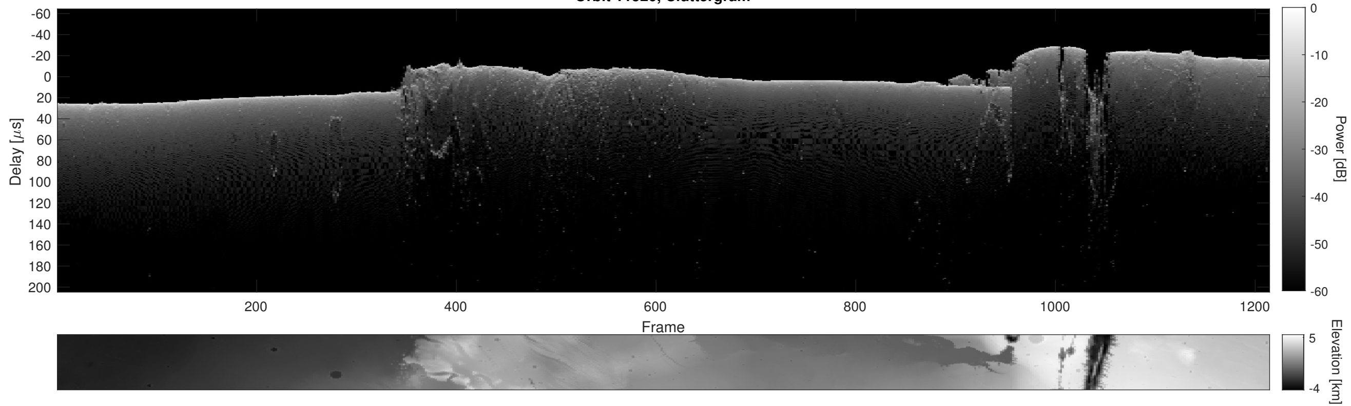
Orbit 11520, Cluttergram
