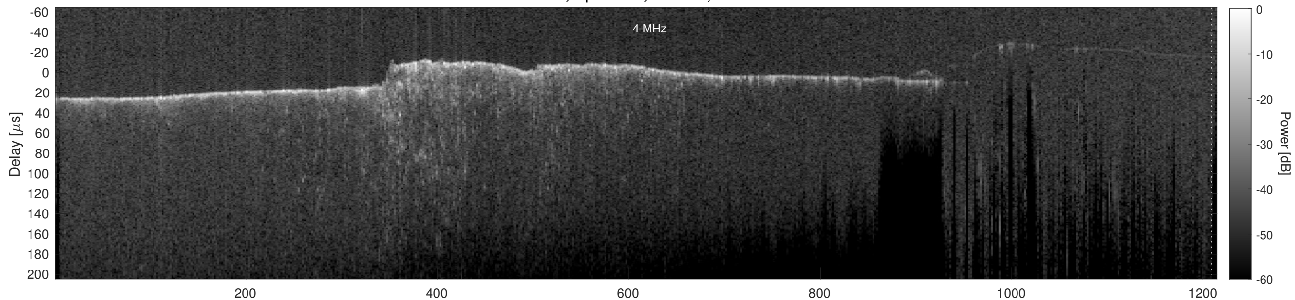
Orbit 11520, Cluttergram
