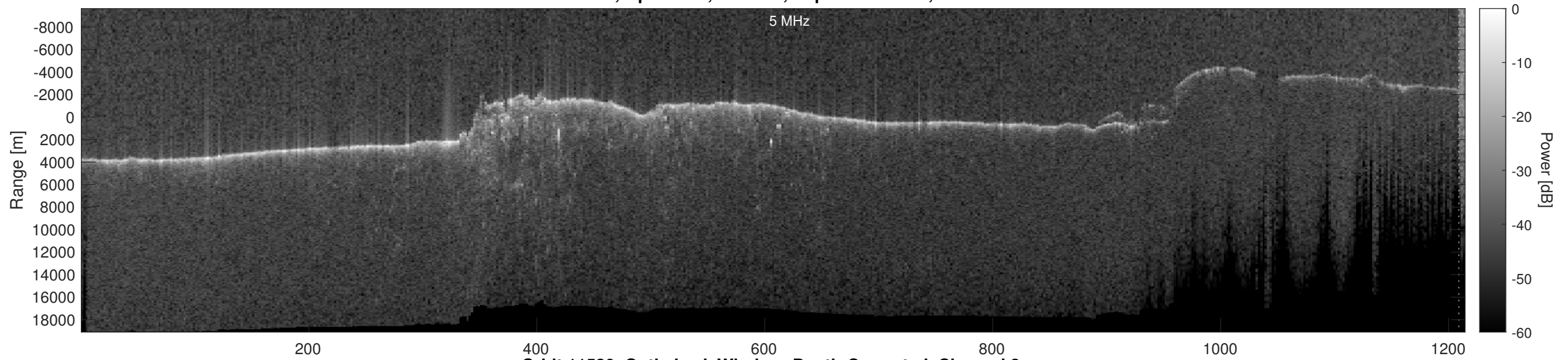
Orbit 11520, Optimized, Window, Depth-Corrected, Channel 2
