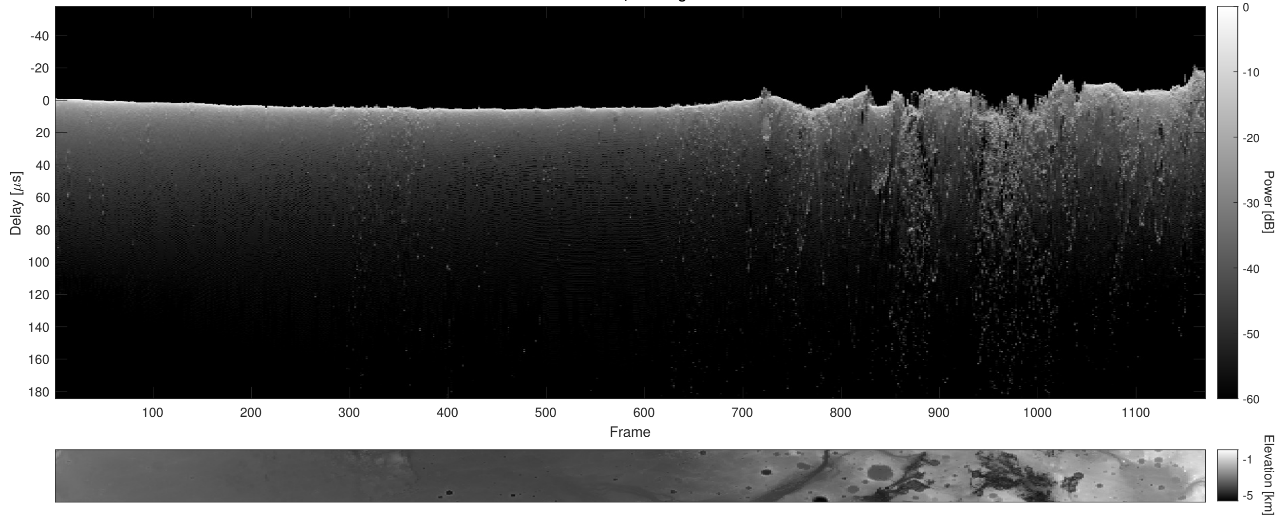
Orbit 11523, Cluttergram
