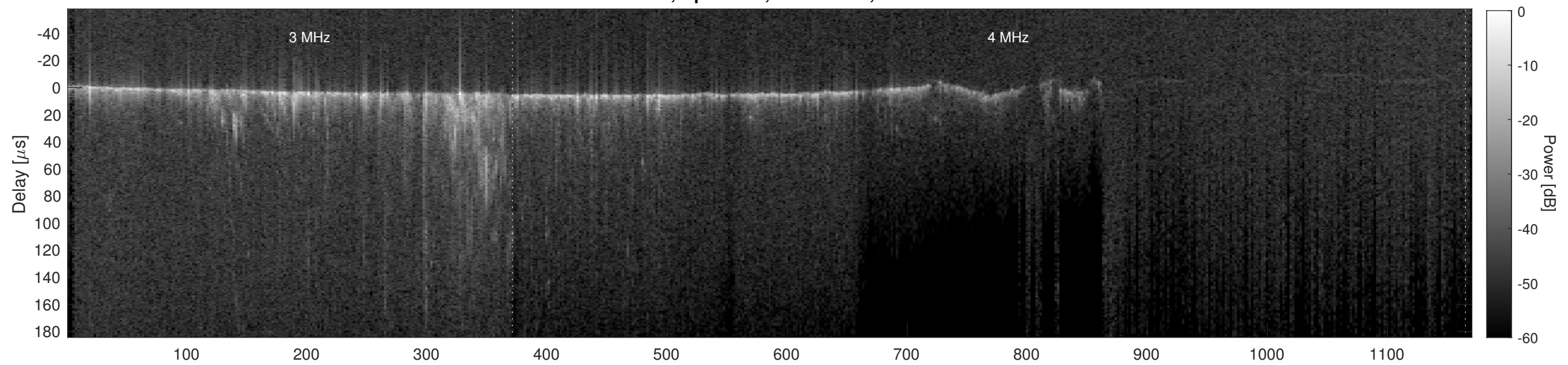
Orbit 11523, Cluttergram
