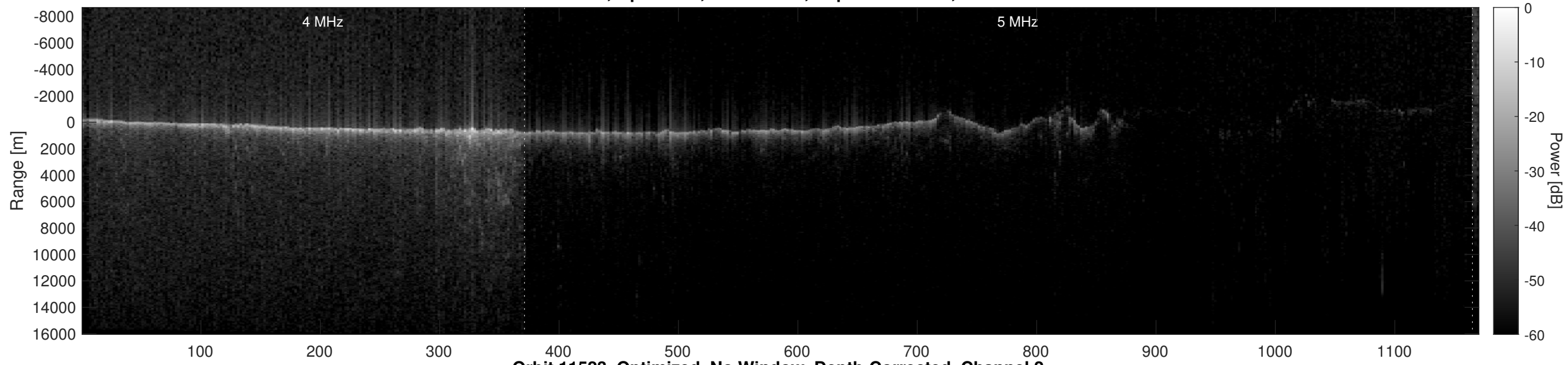
Orbit 11523, Optimized, No Window, Depth-Corrected, Channel 2
