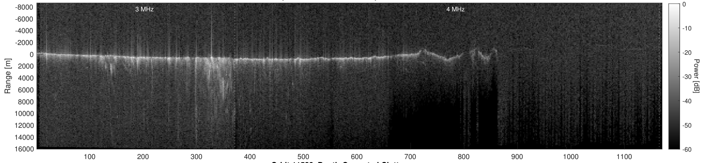
Orbit 11523, Depth-Corrected Cluttergram
