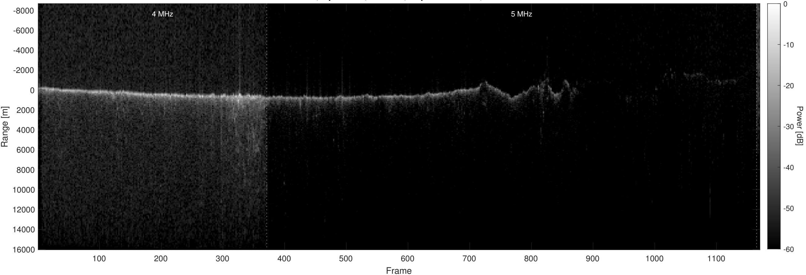
Orbit 11523, Optimized, Window, Depth-Corrected, Channel 2
