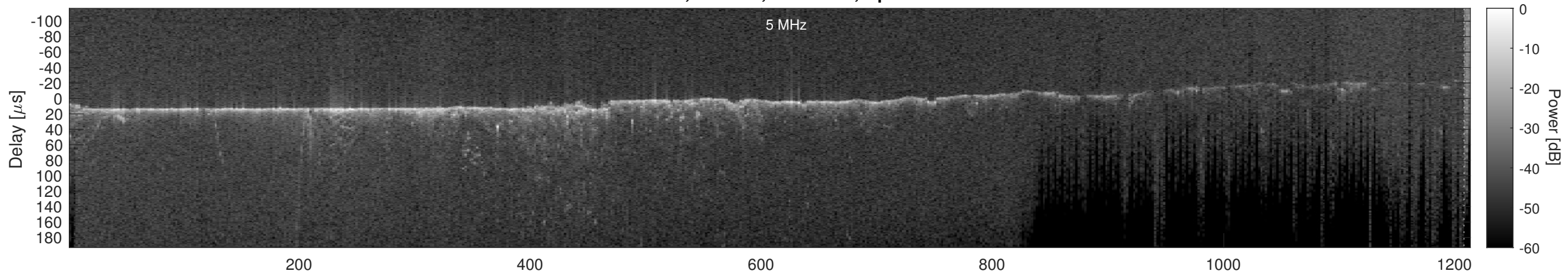
Orbit 11526, Cluttergram
