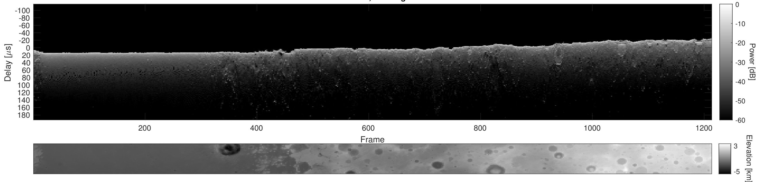
Orbit 11526, Cluttergram
