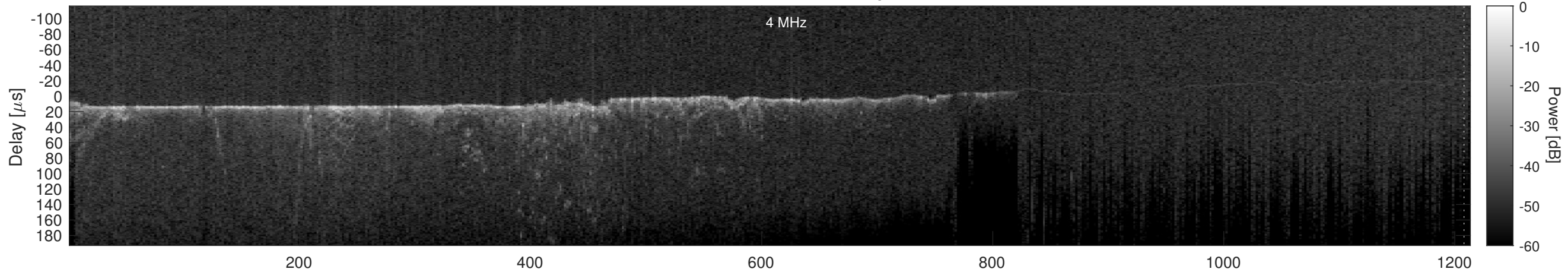
Orbit 11526, Cluttergram
