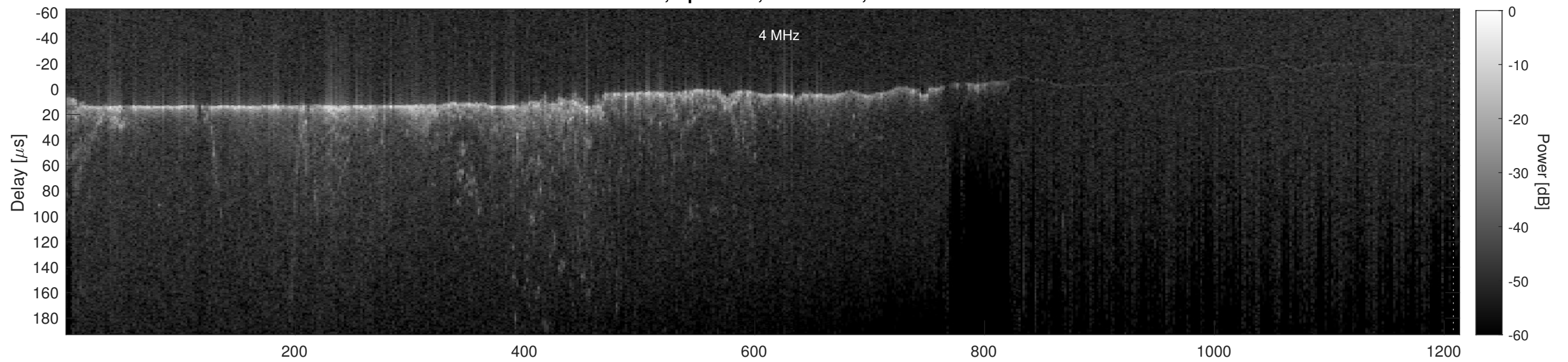
Orbit 11526, Cluttergram
