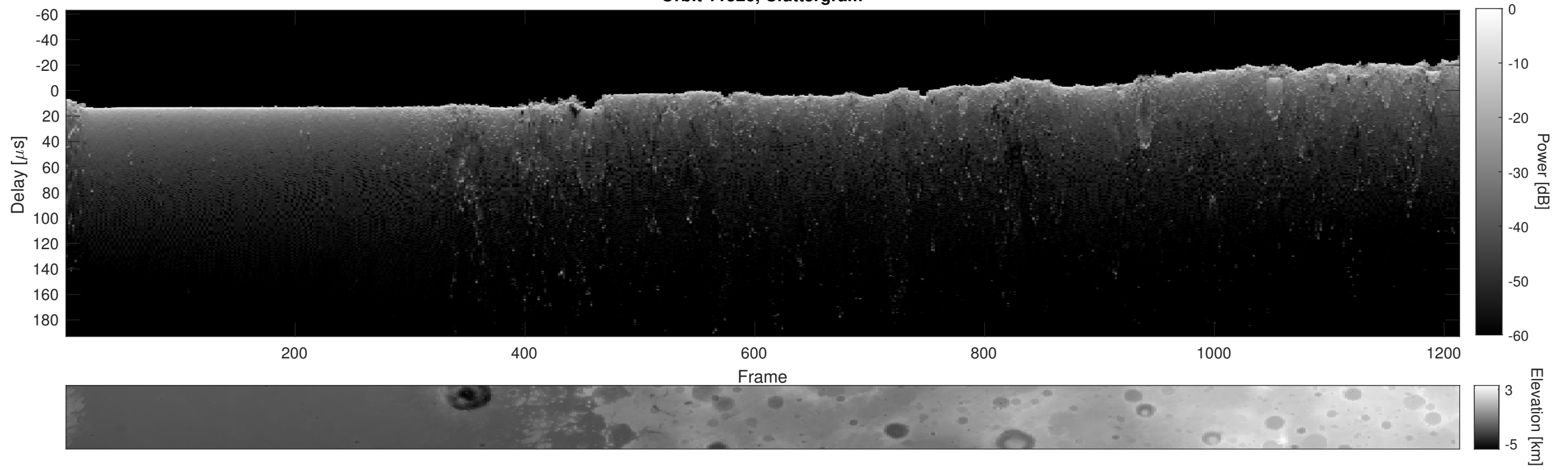
Orbit 11526, Cluttergram
