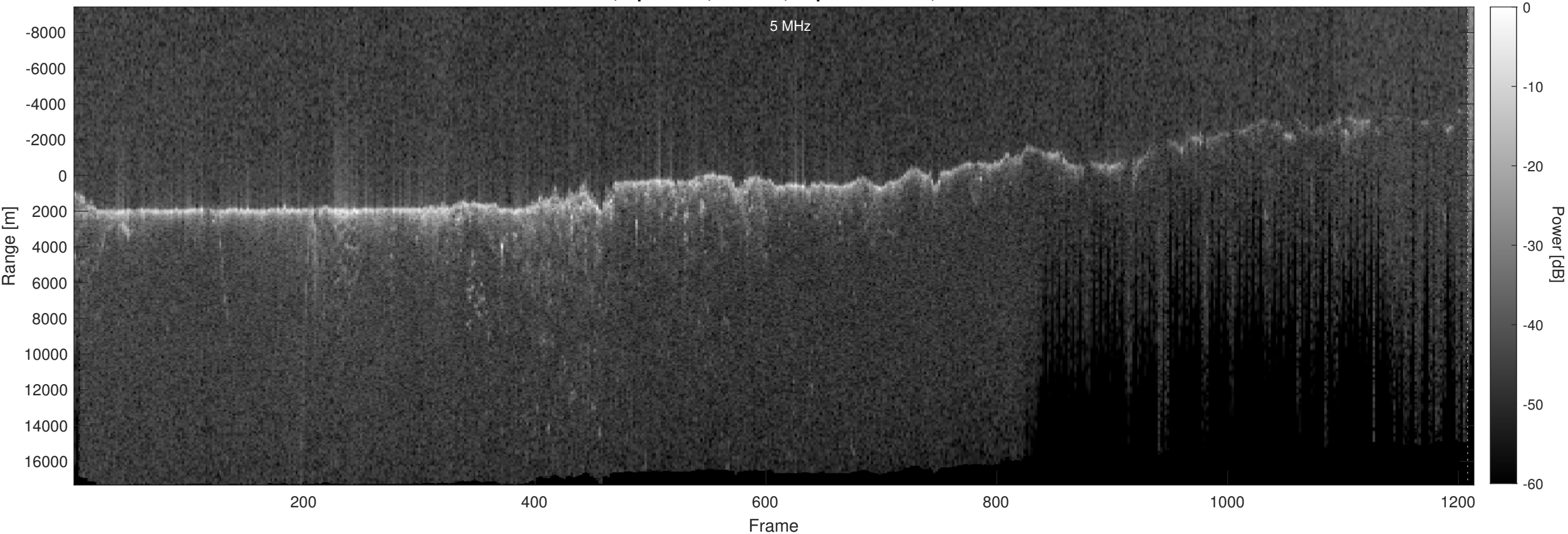
Orbit 11526, Optimized, Window, Depth-Corrected, Channel 2
