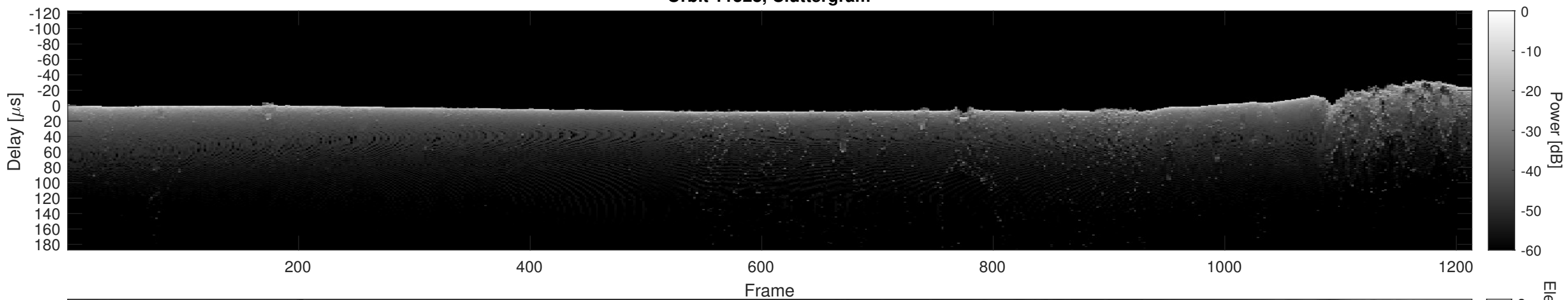
Orbit 11528, Cluttergram
