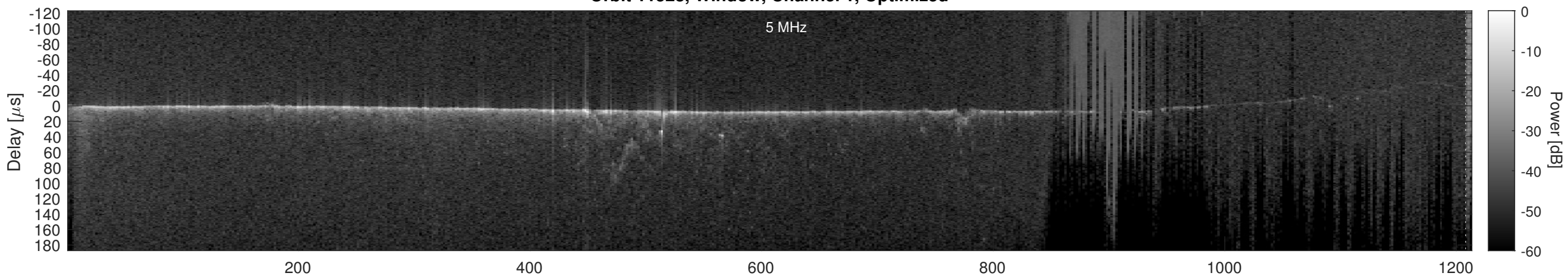
Orbit 11528, Cluttergram
