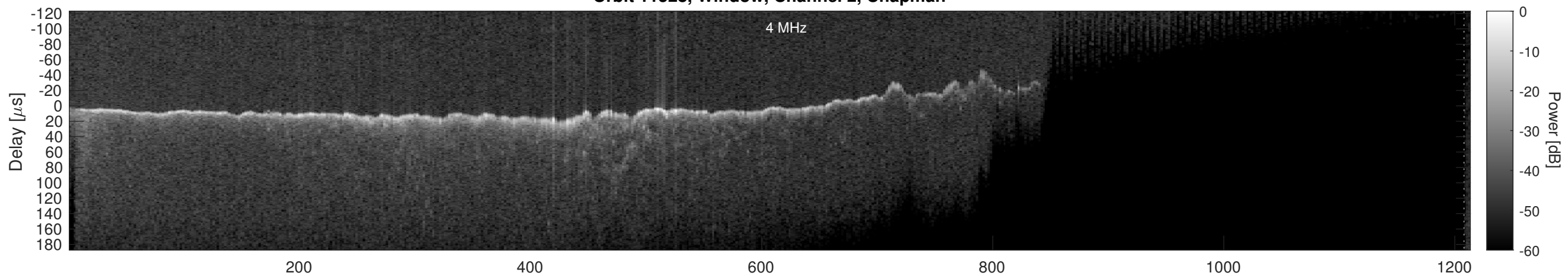
Orbit 11528, Window, Channel 2, Optimized
