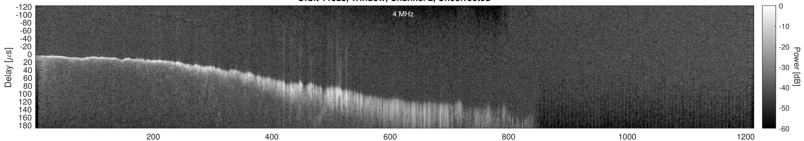
Orbit 11528, Window, Channel 2, Chapman
