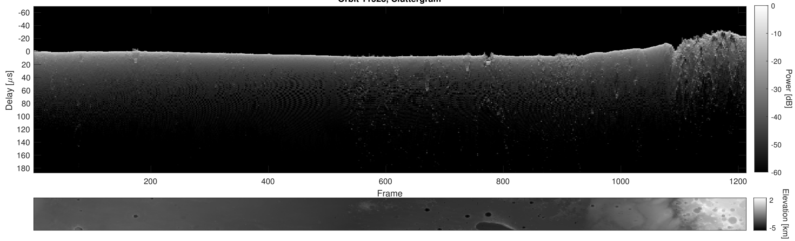
Orbit 11528, Cluttergram
