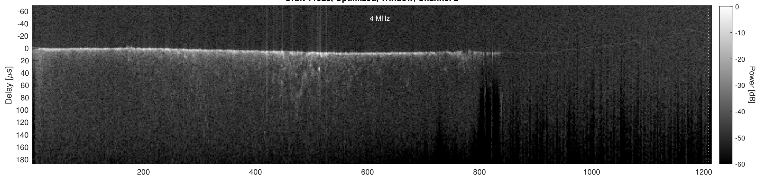
Orbit 11528, Cluttergram
