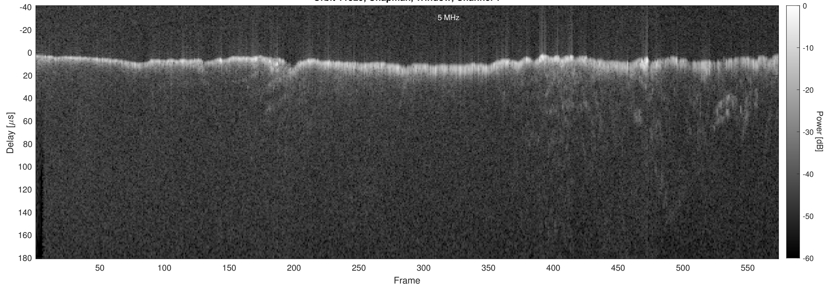
Orbit 11529, Chapman, Window, Channel 2
