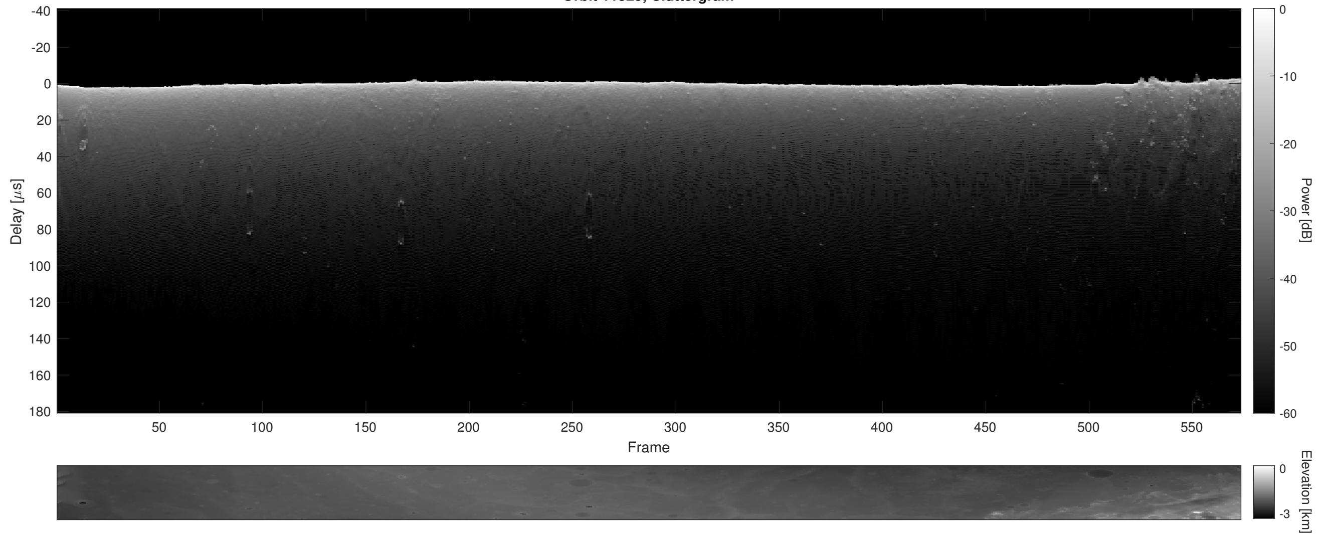
Orbit 11529, Cluttergram
