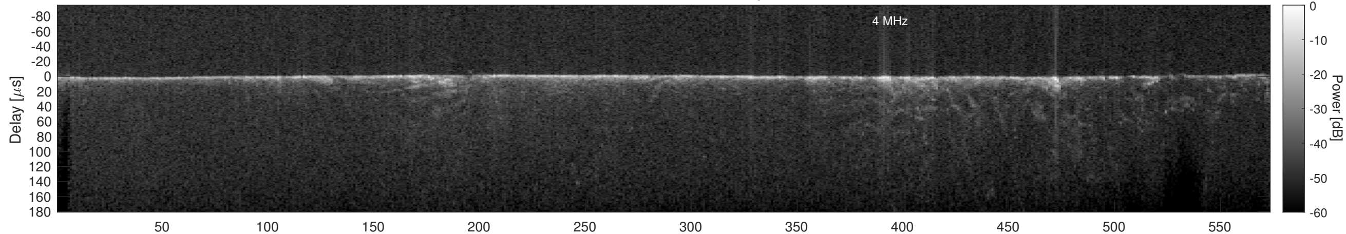
Orbit 11529, Cluttergram
