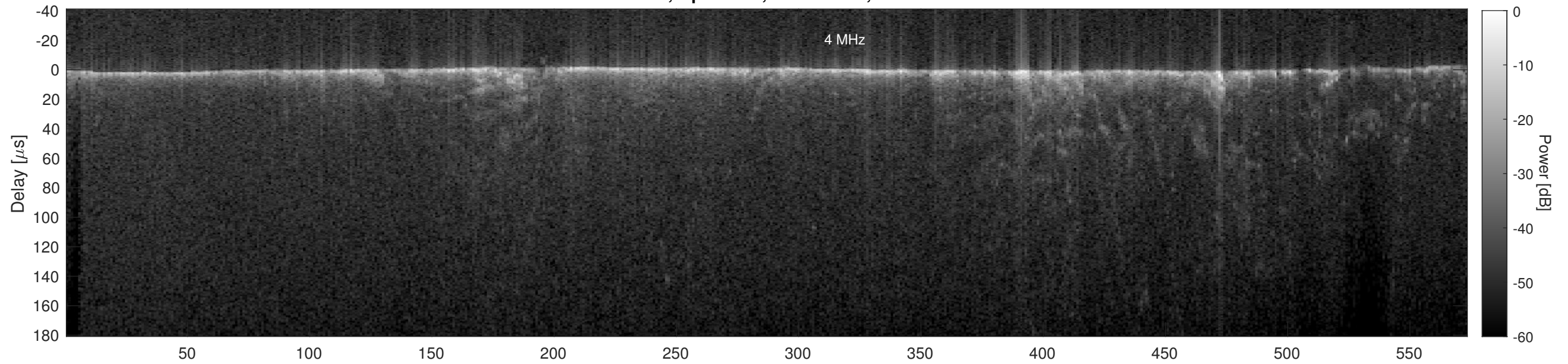
Orbit 11529, Cluttergram
